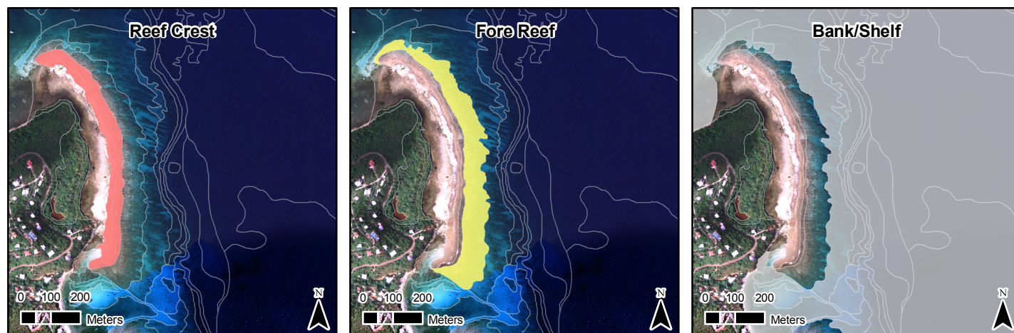
Figure 1.12. A series of orthophotographs illustrating the transition from Reef Crest to Fore Reef to Bank/Shelf zones at Lagoon Point. Each zone is depicted in color on the respective map.
