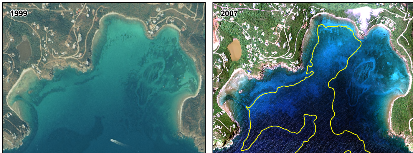
Figure 4.5. Imagery time-series of Rendezvous Bay depicting growth of seagrass beds between 1999 (left) and 2007 (right). The yellow polygon outlines the area of new seagrass growth.
