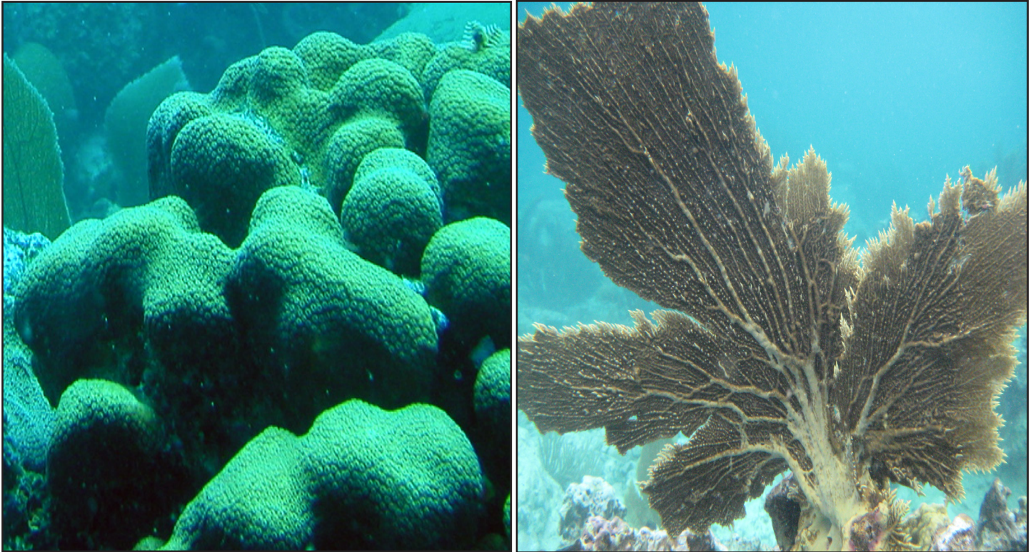
Figure 1.35. Both scleractinian and octocorals are considered when defining live coral cover. Typical corals of St. John include the scleractinian boulder coral ( Montastraea annularis ) and several octocorals including sea fans ( Gorgonia sp.).
