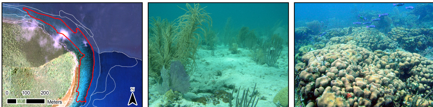
Figure 1.30. In some instances, Live Coral may be the dominant biological cover on St. John's habitats. Underwater pictures display both homogenous octocoral and scleractinian coral dominated environments. A red polygon outlines the feature on orthophotography.
