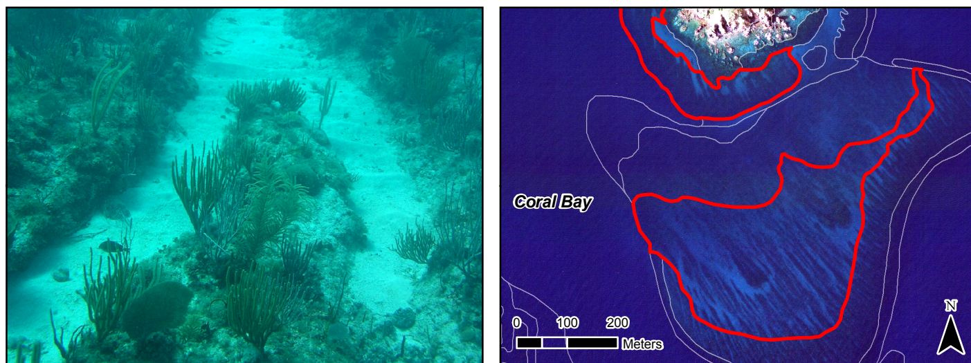
Figure 1.20. Depictions of Pavement with Sand Channels off Turner Point in Coral Bay. A red polygon outlines the feature on orthophotography.
