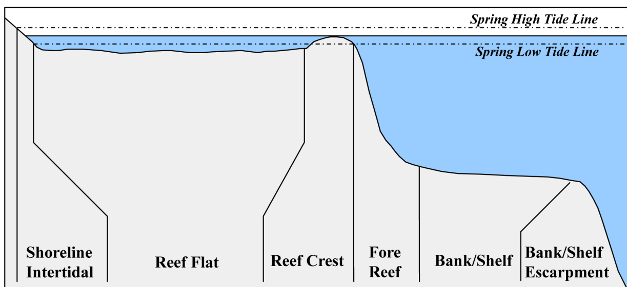
Figure 1.5. Cross-section of zone types where a fringing reef is present. Reef platform is continuous with the shore.
