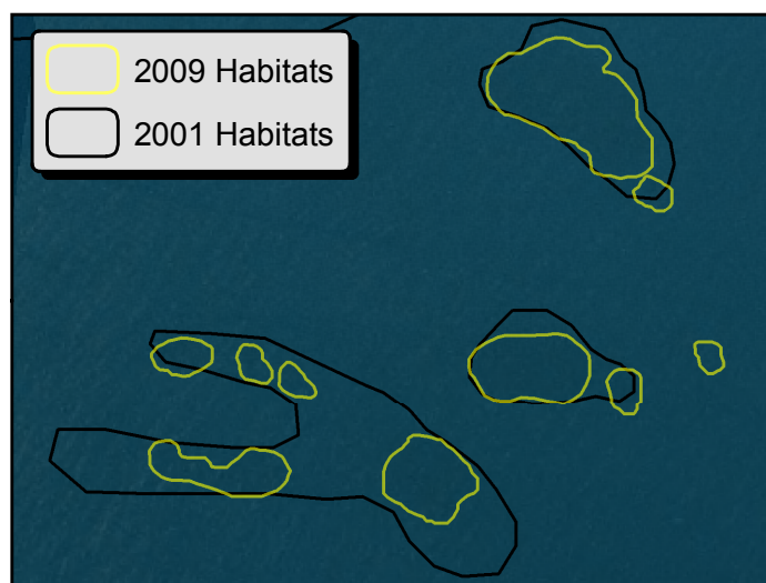
Figure 4.4. Comparison of 2001 and 2009 NOAA habitat boundaries to illustrate the influence of minimum mapping unit on the delineation of patch reefs outside of Reef Bay.
