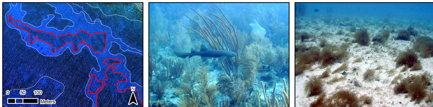
Figure 1.19. Several views of Pavement structure in St. John. The overhead representation outlined by red polygons illustrates the often irregular shape. Also, Pavement may be colonized by a variety of marine flora.
