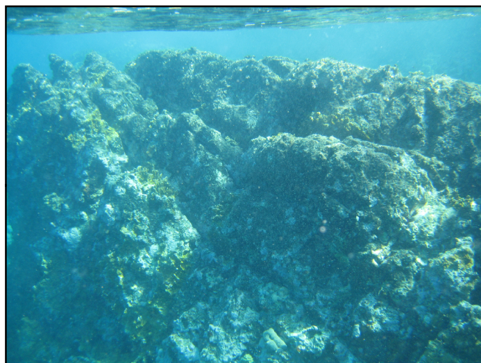
Figure 1.14. Depictions of Rock Outcrop structure on the west side of the mouth of Hawksnest Bay. A red polygon outlines the feature on orthophotography.
