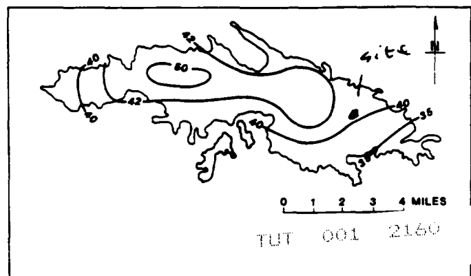
FIGURE 7. Average-annual rainfall, in inches. (Prepared by R.J. Calvesport, (NWS) NOAA.)
