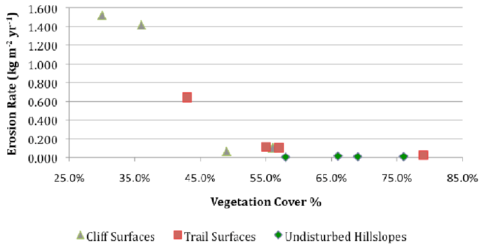
Figure 6 Erosion rates by surface types and % vegetation cover
