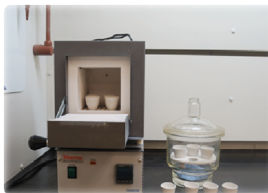
Figure 3 Muffle furnace used for LOI 550 analysis
