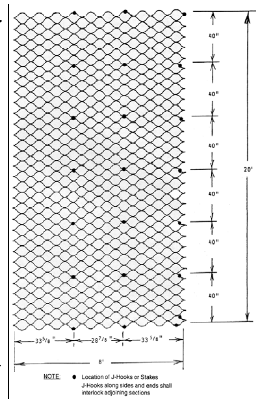
Figure 31. EnviroGrid® light density staking diagram (AGH Industries, Inc., 1999).
