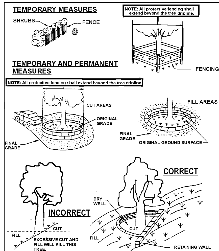
Figure 2. Tree protection practices (Maryland Department of the Environment, 1994).
