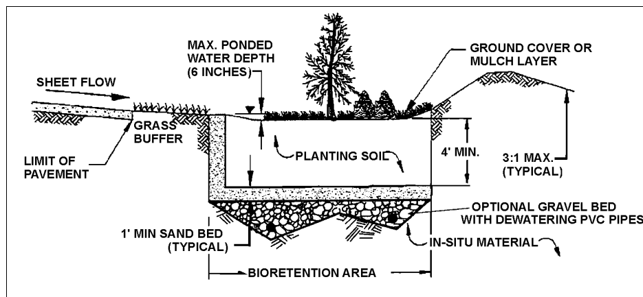
Figure 35. Off-line rain garden cross-section (CH2M Hill, 1998).
