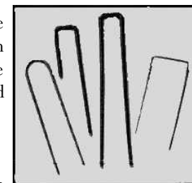
Figure 15. Different types of staples used to anchor erosion control mats.
