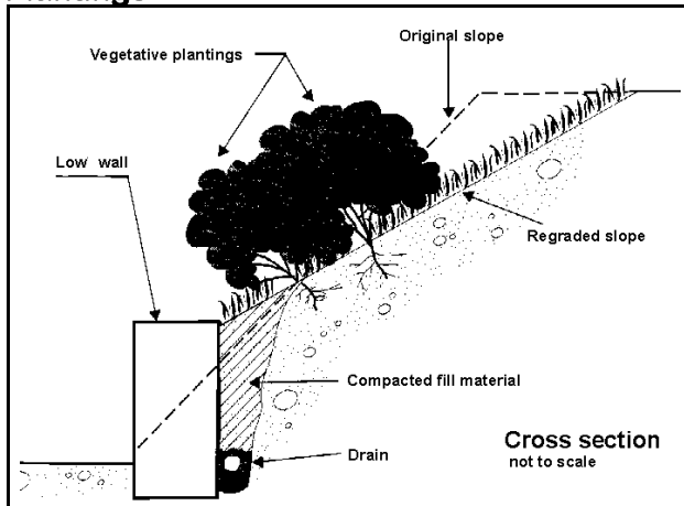
Figure 14. A low wall with plantings above (USDA-SCS, 1992).
