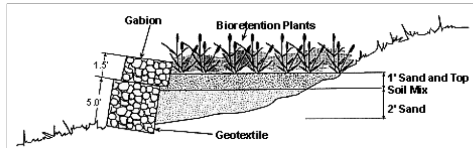
Figure 34. Cross section of an on-line rain garden formed by damming a grass swale with a mild to moderate slope with gabion baskets (CH2M Hill, 1998).
