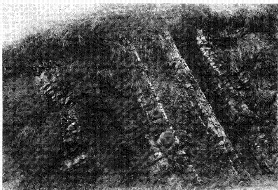
FIG. 14.— Diorite porphyry sills intruded between layers of shales and ashes at K 20, Comerio Road
