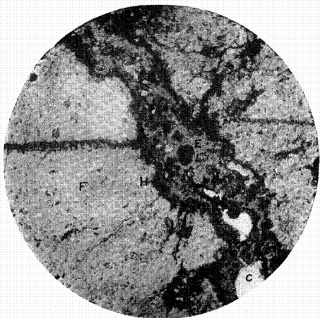
FIG. 21.— Latite, showing veins filled with epidote and iron oxides
