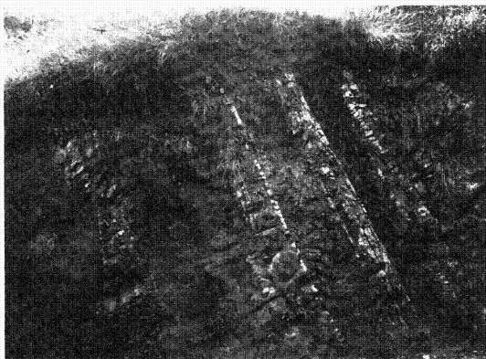
FIG. 1.— Diorite porphyry sills
