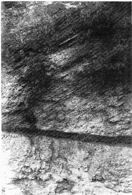
FIG. 26.— Cross-bedded structure in the San Juan formation at Arecibo
