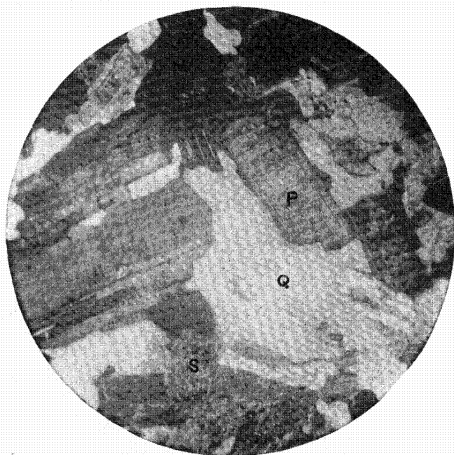
FIG. 18.— Soda granite occurring south of Naranjito
