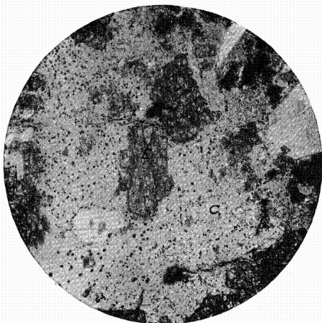
FIG. 16.—Photomicrograph of vitrophyr occurring north of Cidra
