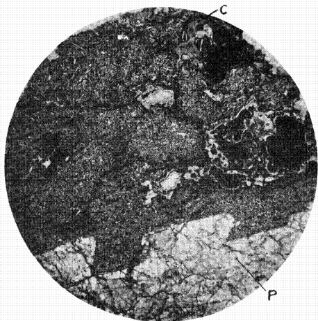
FIG. 23.— Andesite porphyry impregnated with chrysocolla. Barrio Pasto
