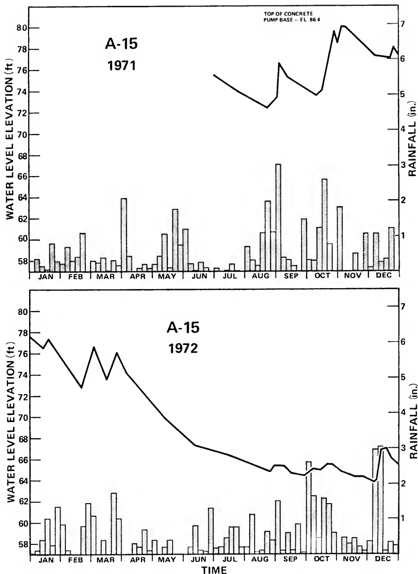
Figure G-1. Water levels in well A-15, 1971-1972.
