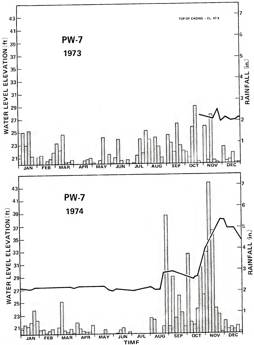
Figure G-27. Water levels in well PW-7, 1973-1974.
