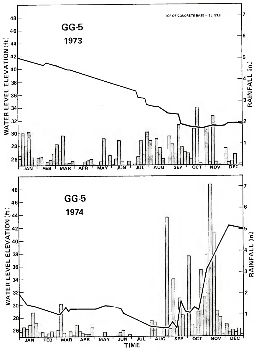
Figure G-12. Water levels in well GG-5, 1973-1974.
