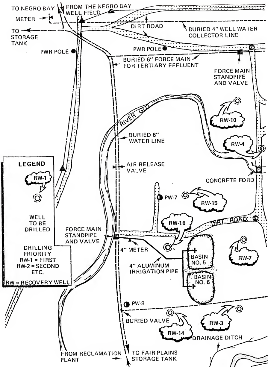
Figure 39. Future well field development in the Golden Grove recharge area.
