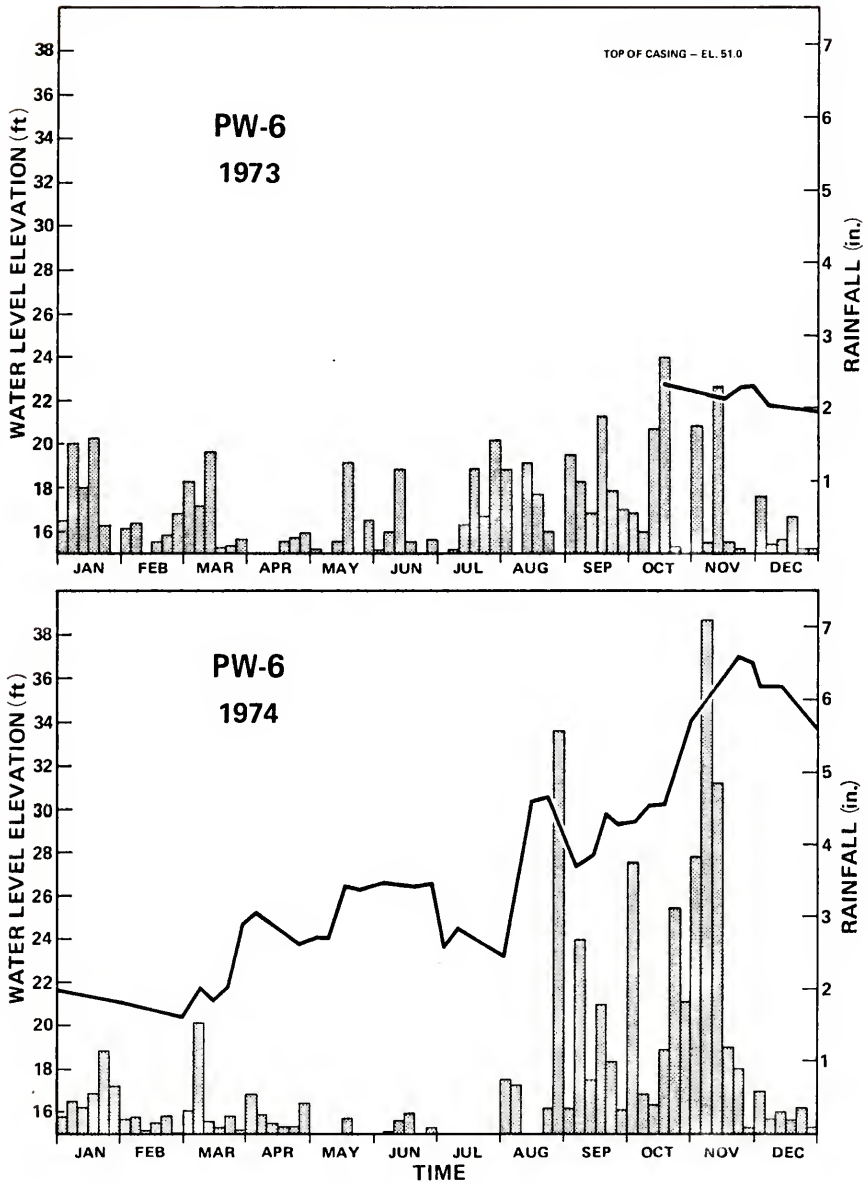
Figure G-25. Water levels in well PW-6, 1973-1974.
