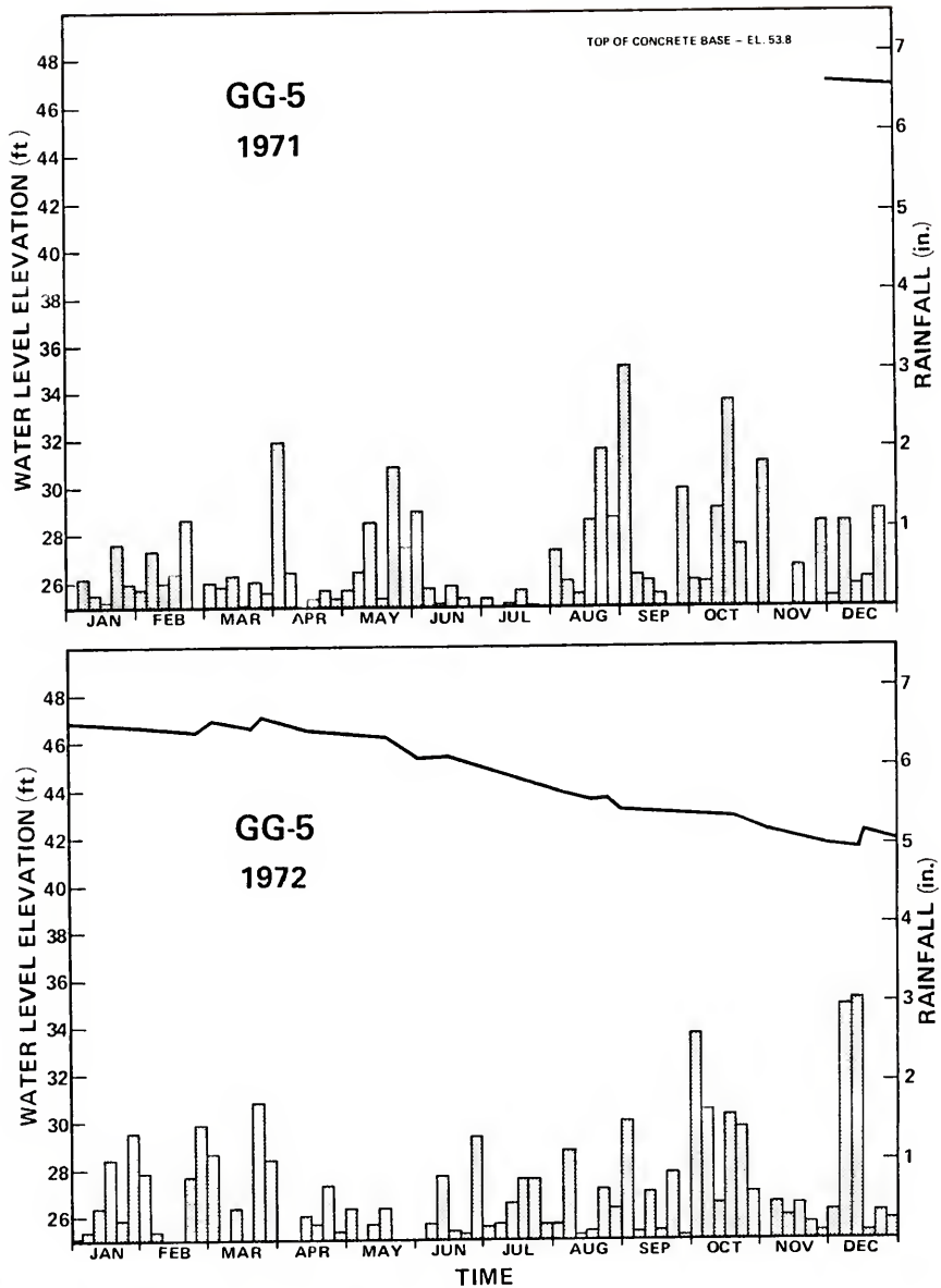
Figure G-11. Water levels in well GG-5, 1971-1972.
