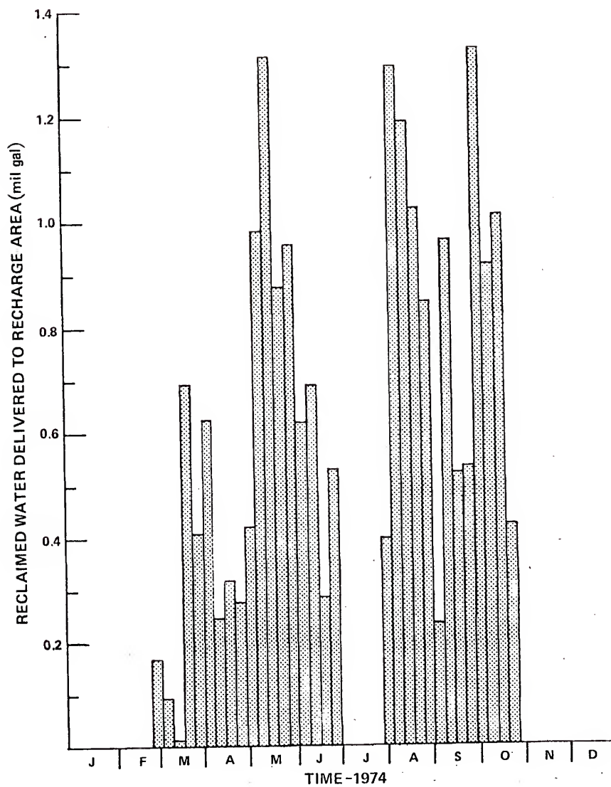
Figure 23. AWWTP production utilized for artificial groundwater recharging.
