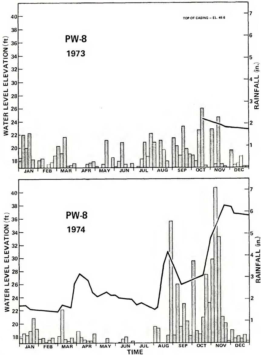
Figure G-29. Water levels in well PW-8, 1973-1974.
