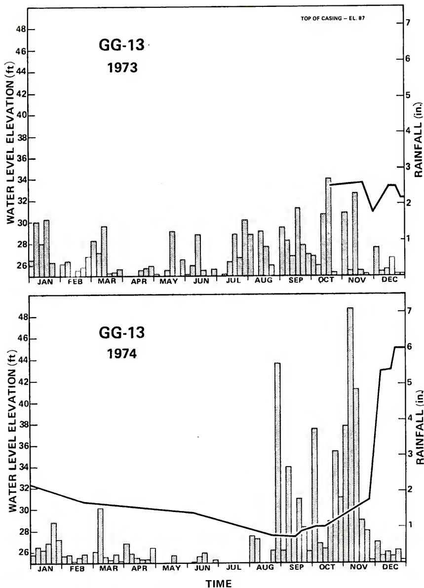
Figure G-17. Water levels in well GG-13, 1973-1974.
