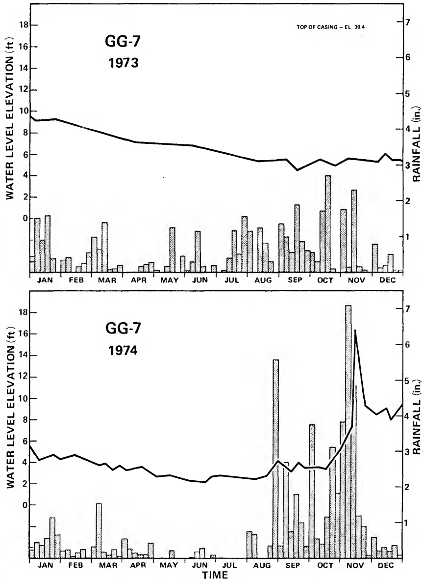
Figure G-15. Water levels in well GG-7, 1973-1974.
