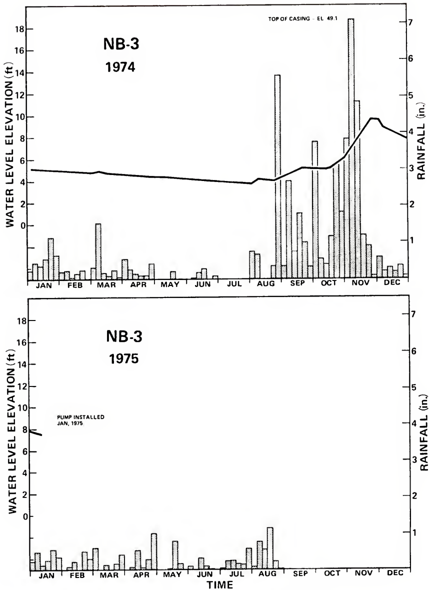
Figure G-19. Water levels in well NB-3, 1974-1975.
