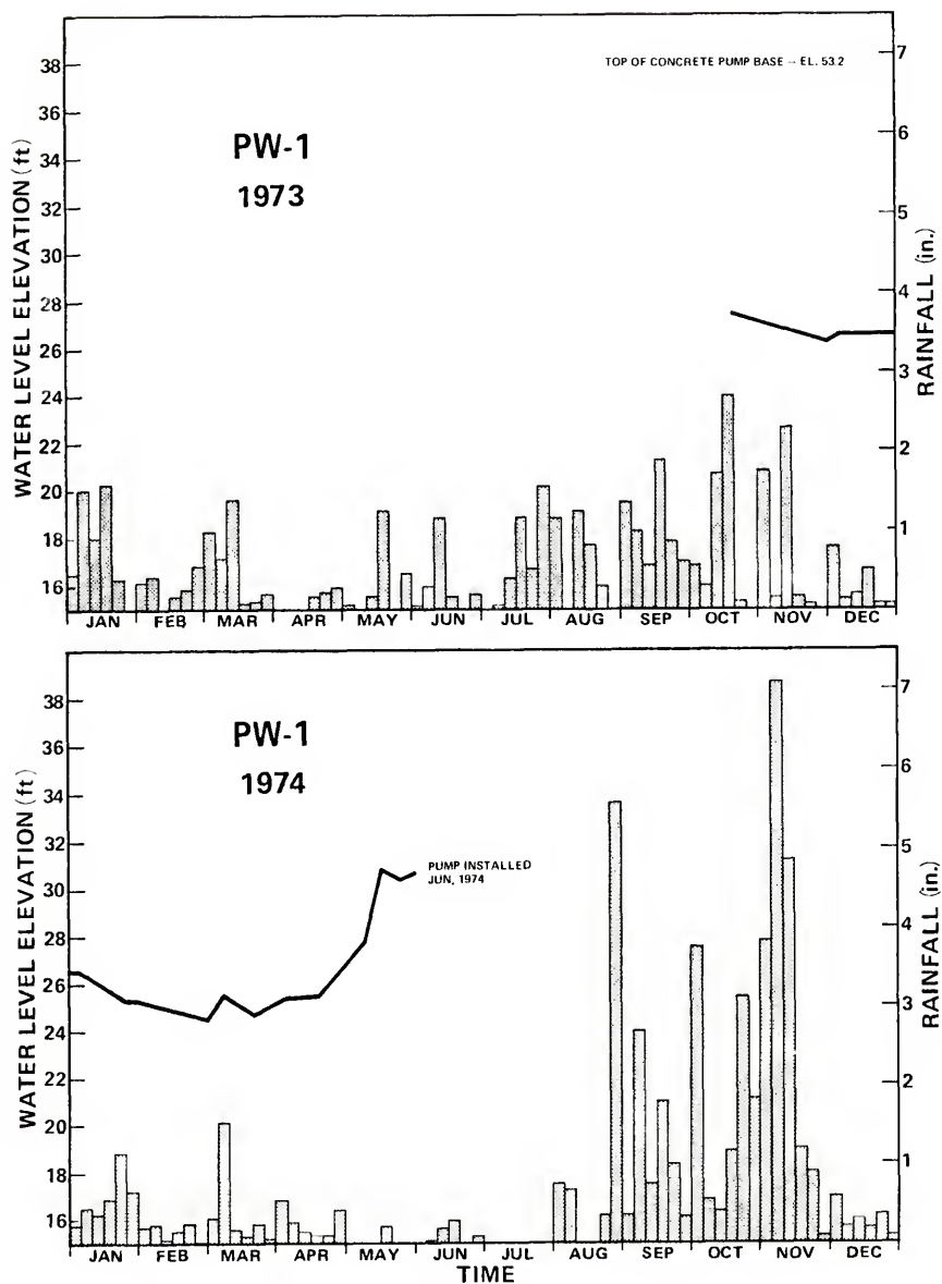
Figure G-20. Water levels in well PW-1, 1973-1974.
