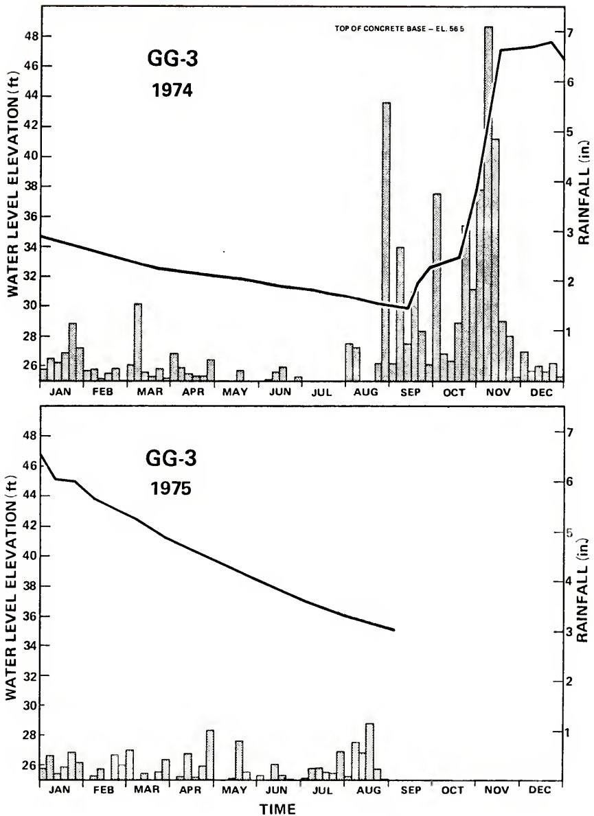
Figure G-9. Water levels in well GG-3, 1974-1975.
