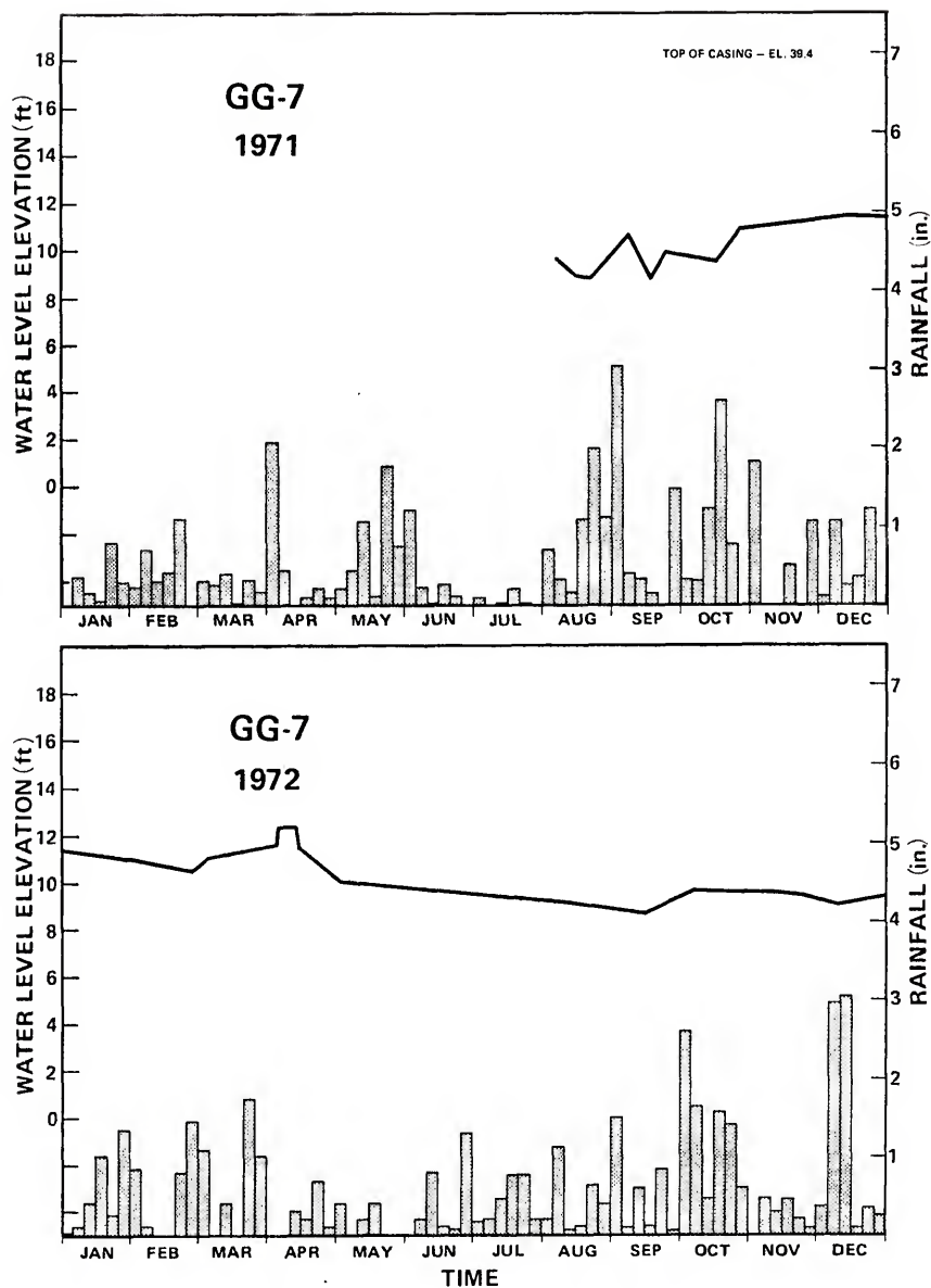
Figure G-14. Water levels in well GG-7, 1971-1972.
