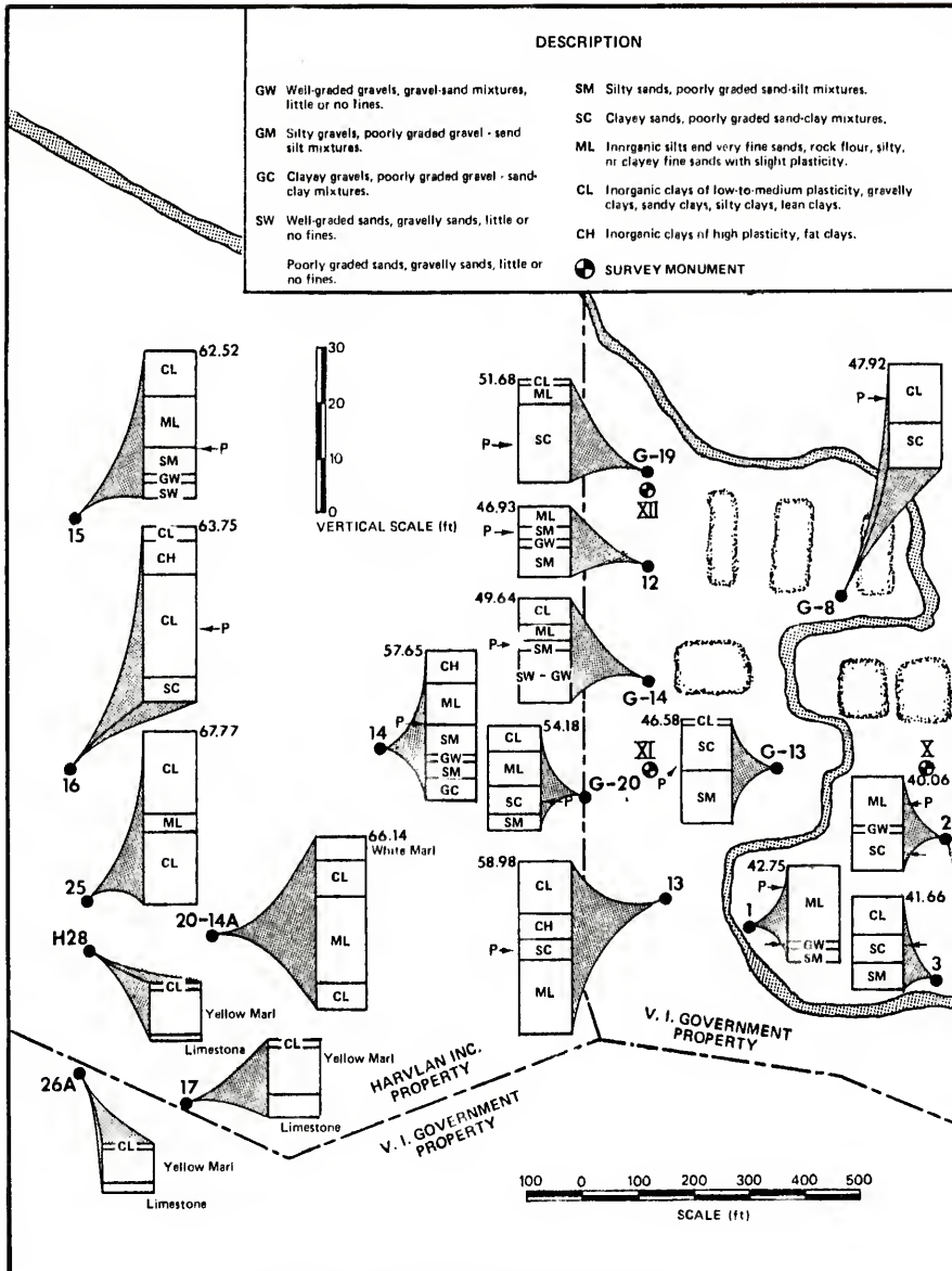
Figure F-1. Soil boring locations in Golden Grove.
