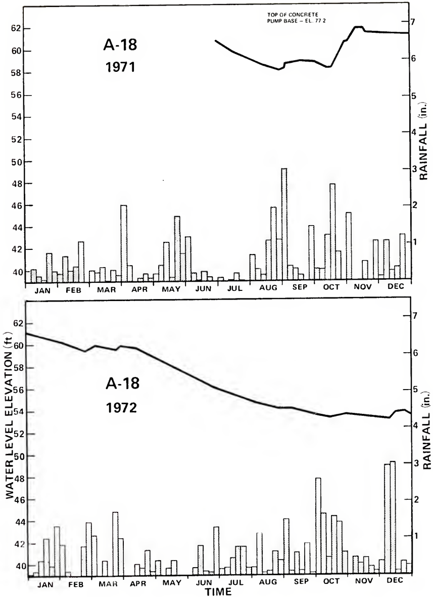
Figure G-4. Water levels in well A-18, 1971-1972.
