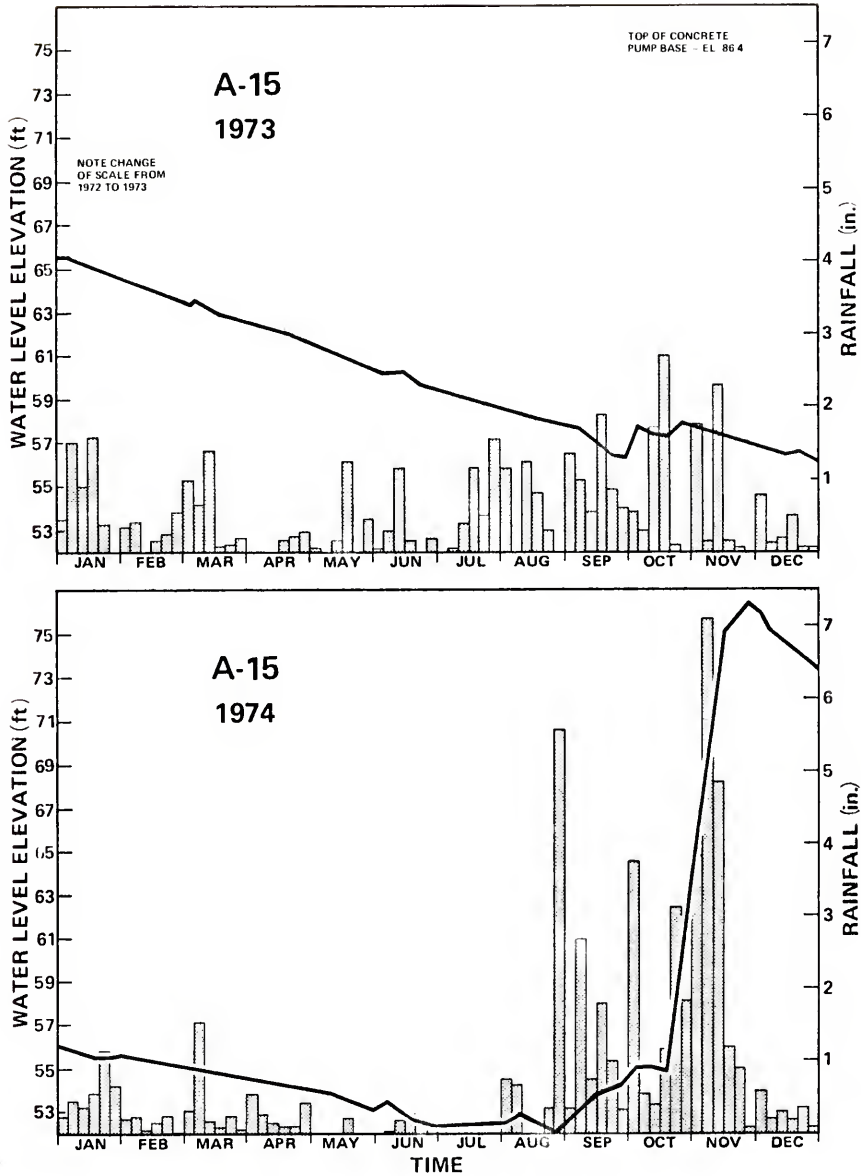
Figure G-2. Water levels in well A-15, 1973-1974.
