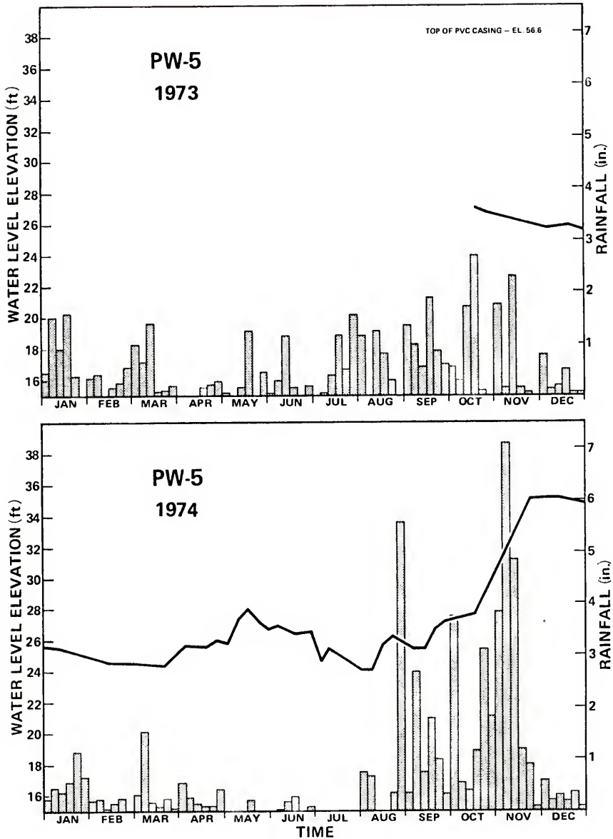
Figure G-23. Water levels in well PW-5, 1973-1974.
