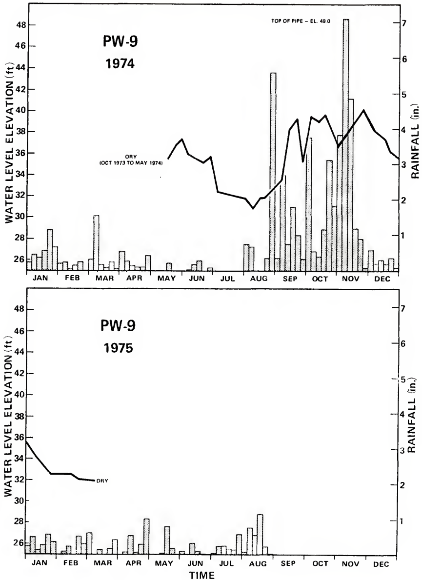
Figure G-31. Water levels in well PW-9.
