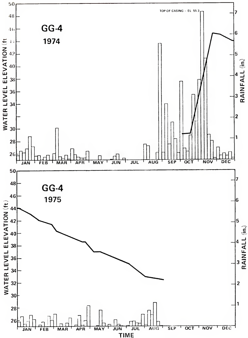
Figure G-10. Water levels in well GG-4, 1974-1975.
