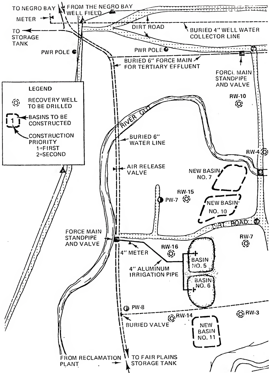
Figure 40. Future expansion of the spreading basins in the Golden Grove recharge area.
