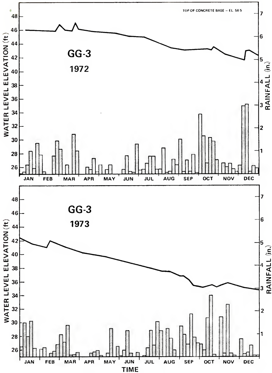
Figure G-8. Water levels in well GG-3, 1972-1973.
