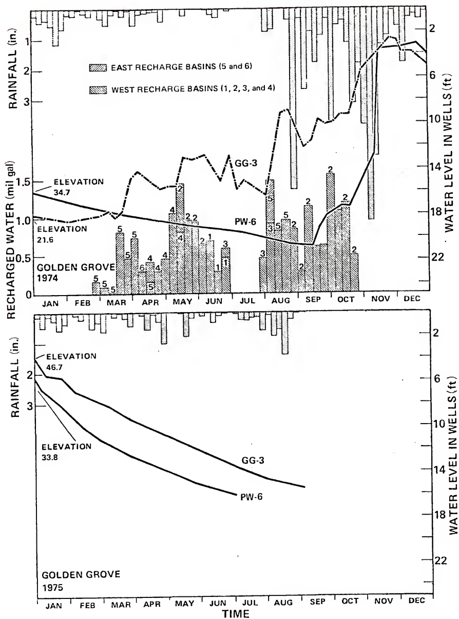
Figure 33. Comparison of wells GG-3 and PW-6, 1974-1975.
