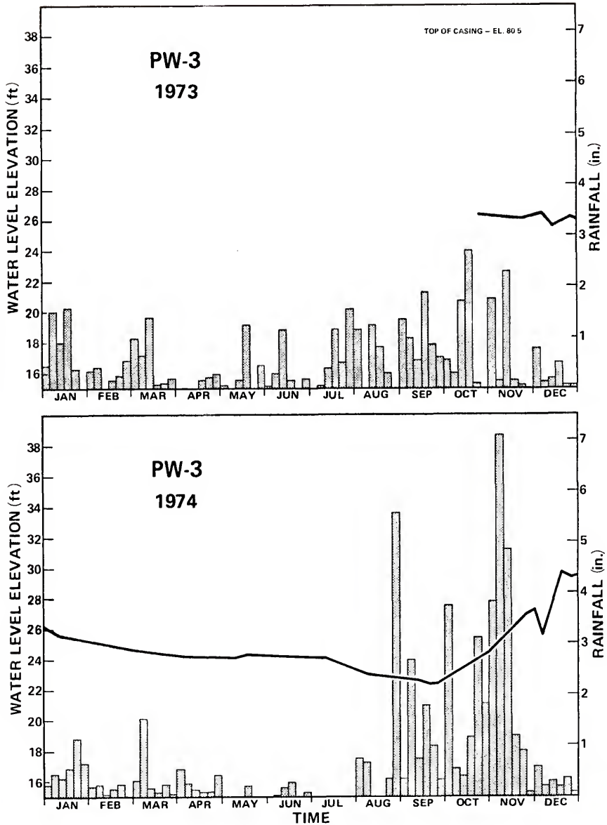
Figure G-21. Water levels in well PW-3, 1973-1974.
