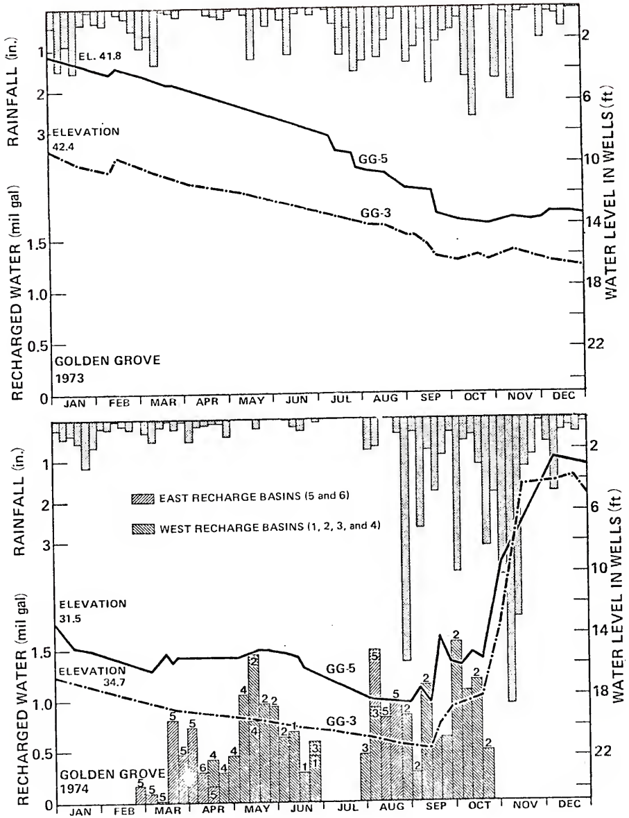
Figure 31. Comparison of wells GG-3 and GG-5, 1973-1974.
