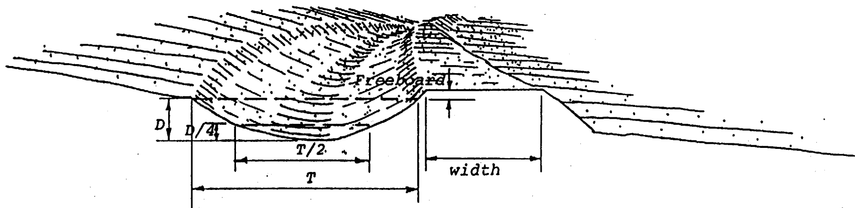
PARABOLIC CROSS-SECTION
