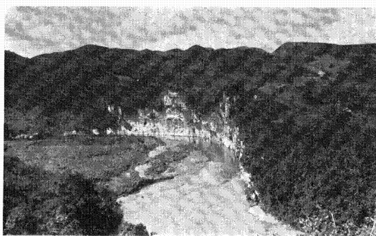
FIG. 14.—The gorge of the Manatí, incised below the surface of the coastal plain
