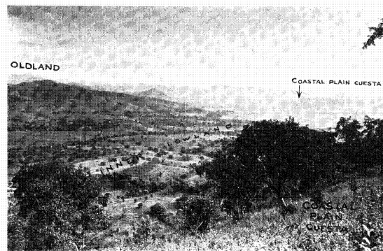
FIG. 17.—The inner lowland of the south coast, looking eastward from cuesta face back of Ponce
