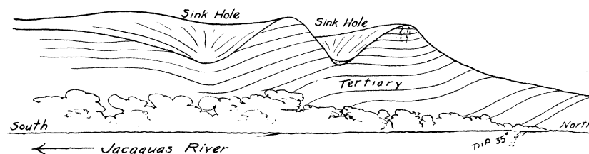
FIG. 22.—Section of hill along Jacaguas River one mile southwest of Juana Diaz
