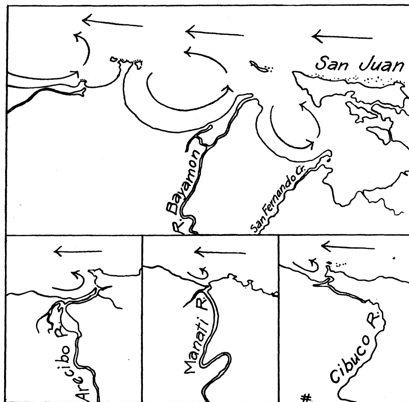
FIG. 35.—River mouths of the north coast
