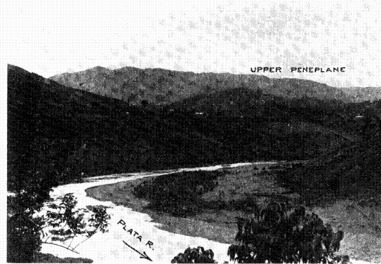
FIG. 25.—The high terrace of the Plata River at K 13 on the Comerio road.
