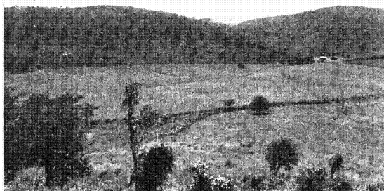
FIG. 6.—Appalachian ridge structure in the oldland rocks between Boqueron and Parguera
