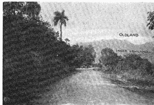
FIG. 20.—Beds of the coastal plain dipping slightly toward the oldland
