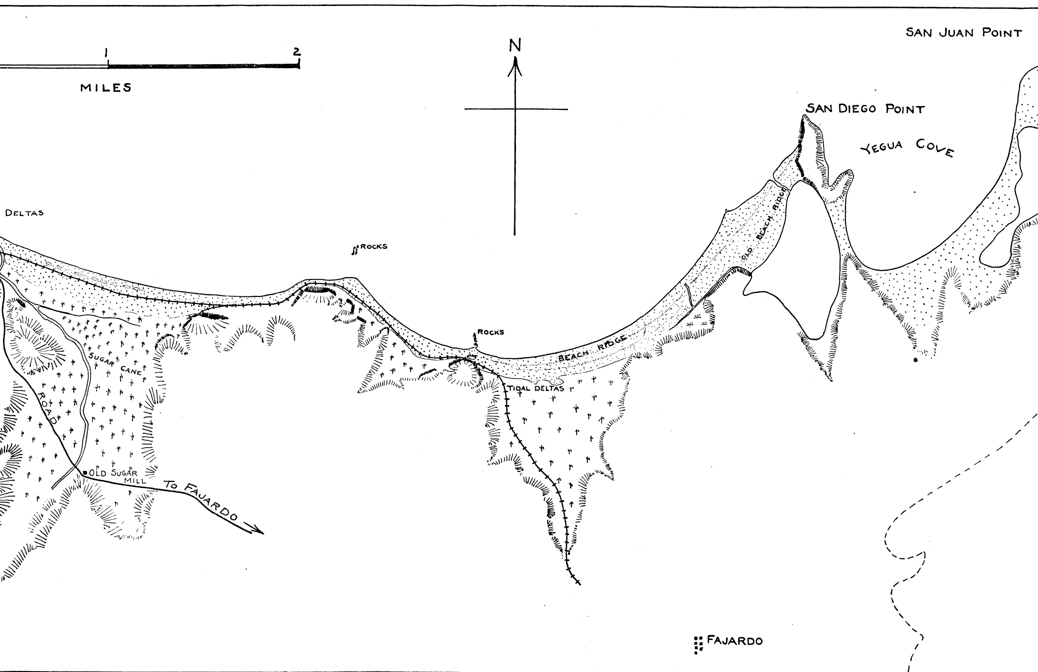
FIG. 27.—Sketch map of the coast east of Luquillo Showing bars built across the mouths of drowned valleys.
