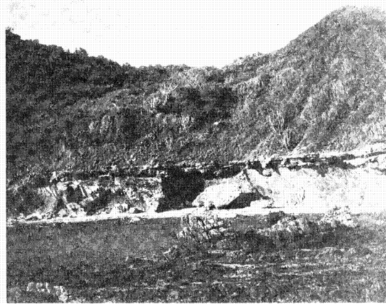
FIG. 37.—The uplifted beach on the south side of Desecheo Island
