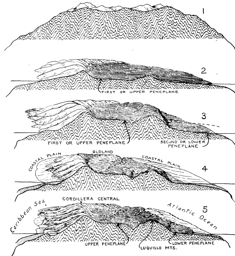
FIG. 4.—The main stages in the physiographic development of Porto Rico
