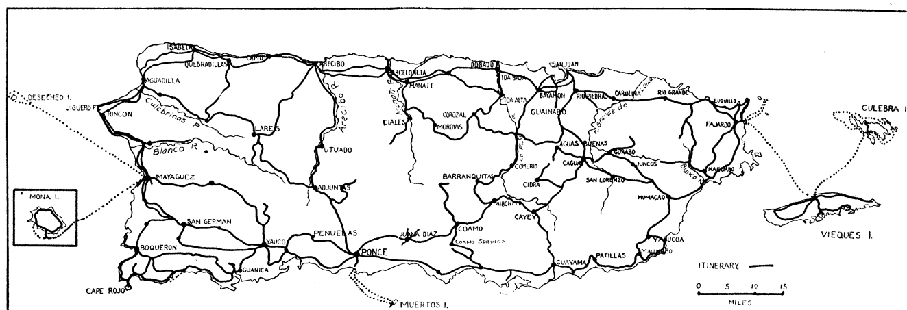
FIG. 2.—Sketch map of Porto Rico showing regions visited
