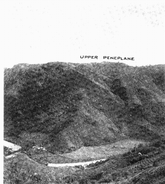
FIG. 7.—Valley of the Manatí River above Ciales
