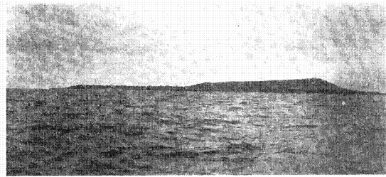
FIG. 41.— Muertos Island from the north
