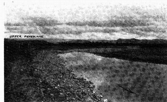
FIG. 24.—Lower course of the Descalabrada River during the dry season.
