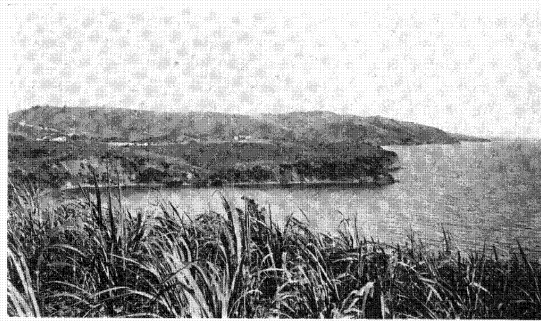
FIG. 23.— The drowned coast of eastern Porto Rico View north of Fajardo, looking toward San Juan Point. Most of the headlands have been cliffed by the waves.
