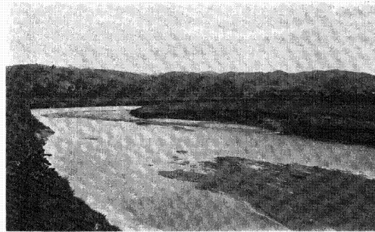
FIG. 8.—The valley and flood plain of the Río Grande de Loíza near Carolina
