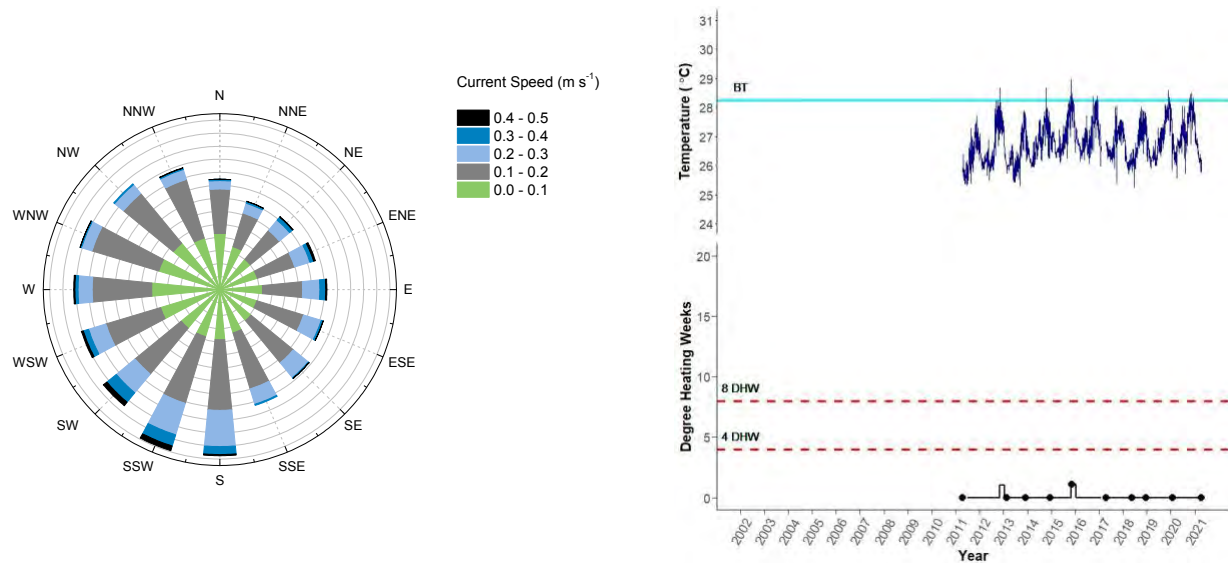
Figure 126. Ginsburgs Fringe current speed (50 m depth) and benthic temperature (63 m depth). BT = bleaching threshold ; DHW = degree heating weeks.
