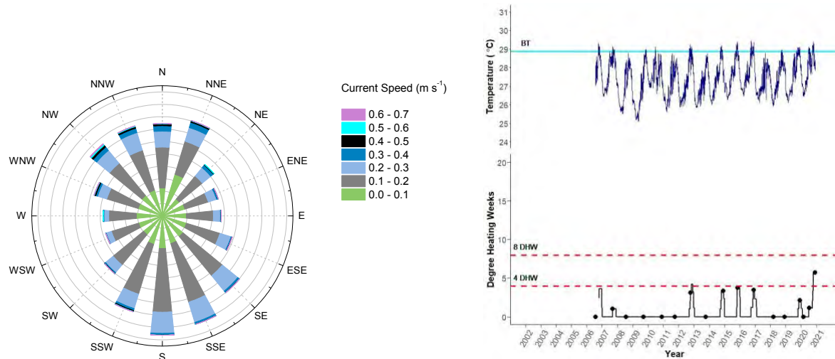
Figure 130. Grammanik Tiger benthic currents speed and temperature record (38 m depth).
