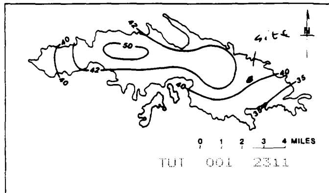
FIGURE 7. Average annual rainfall, in inches. (Prepared by R.J. Calvesbert, (NWS) NOAA.)
