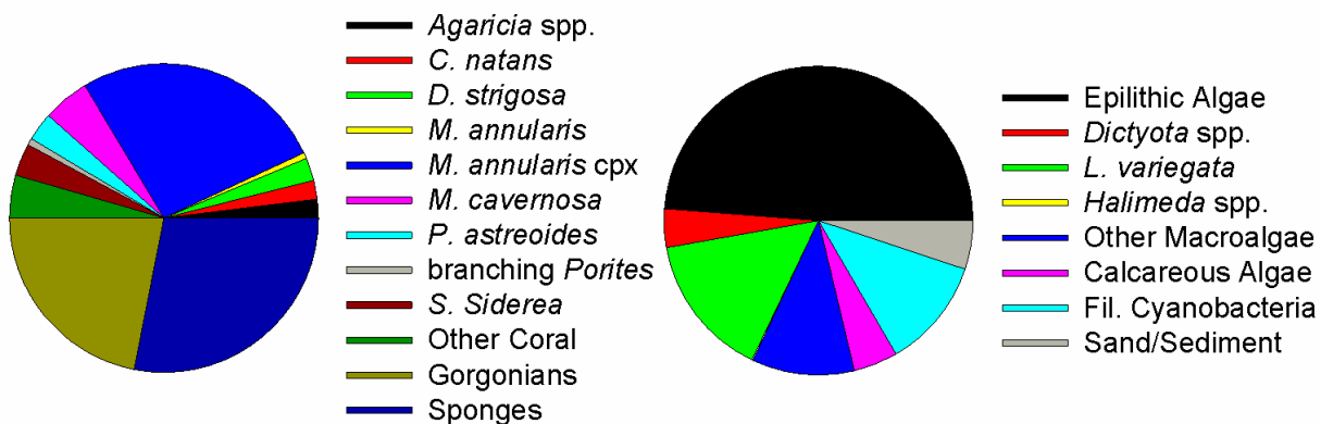
Figure 68. Lang Bank Red Hind FSA (left) Relative composition of the sessile epibenthic animal community. (right) Relative composition of the algal community and unconsolidated sediment.
