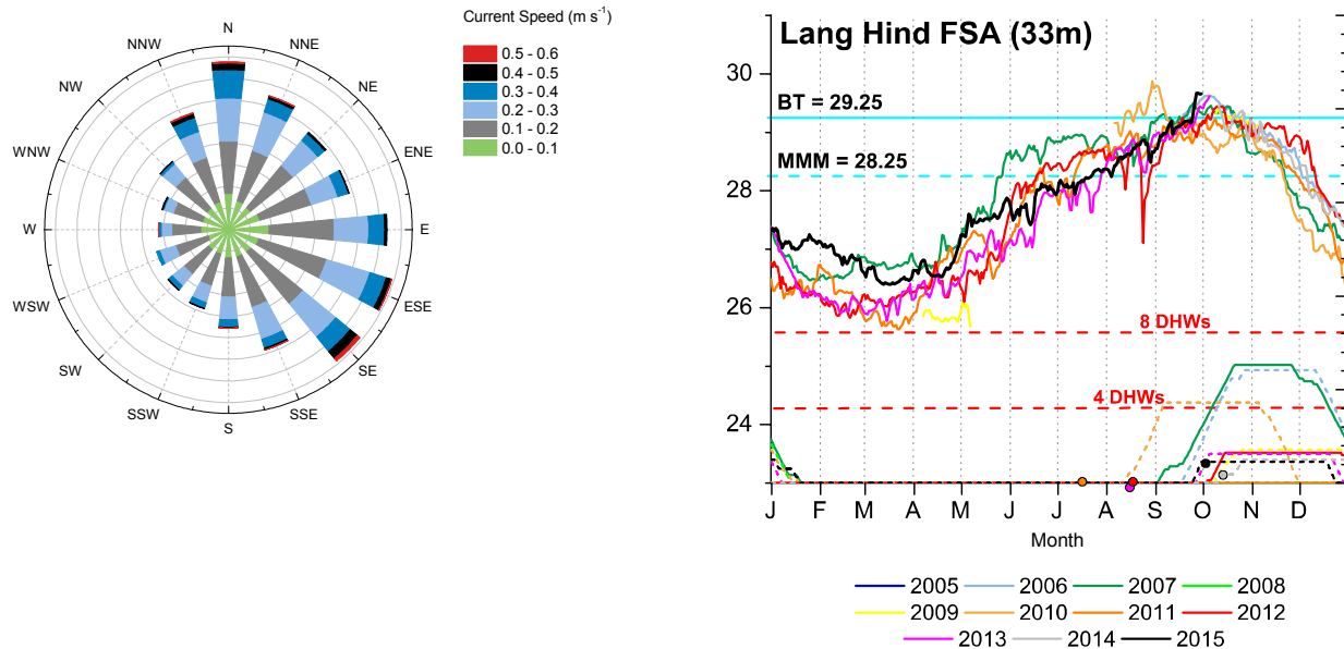
Figure 67. Lang Bank Hind current speed (left) and benthic temperature (right; 33 m depth)
