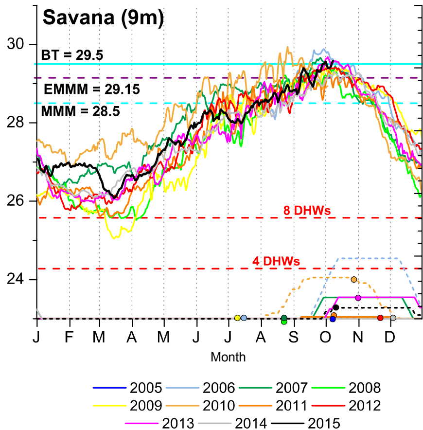
Figure 169. Savana benthic temperature record (10 m depth).
