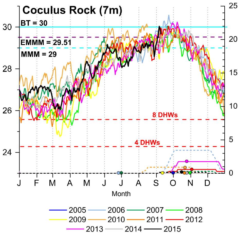
Figure 128. Coculus Rock benthic temperature record (7 m depth).
