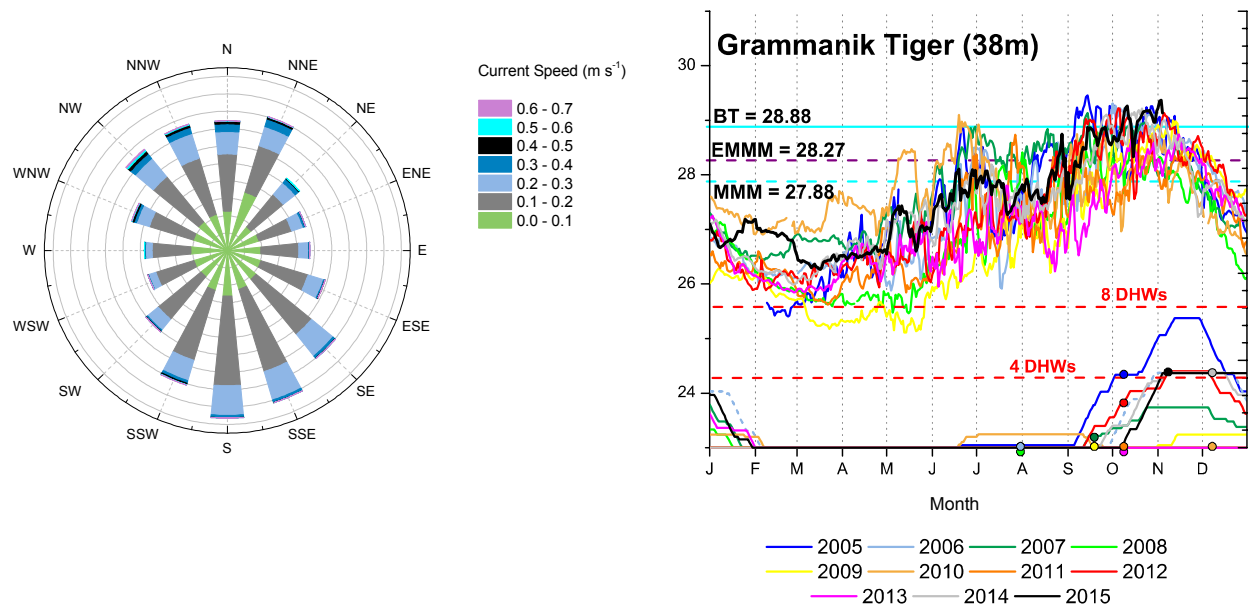
Figure 148. Grammanik Tiger benthic currents speed and temperature record (38 m depth).
