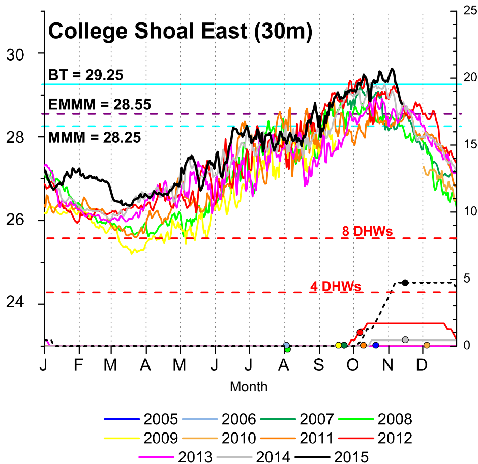
Figure 133. College Shoal benthic temperature record (29 m depth).
