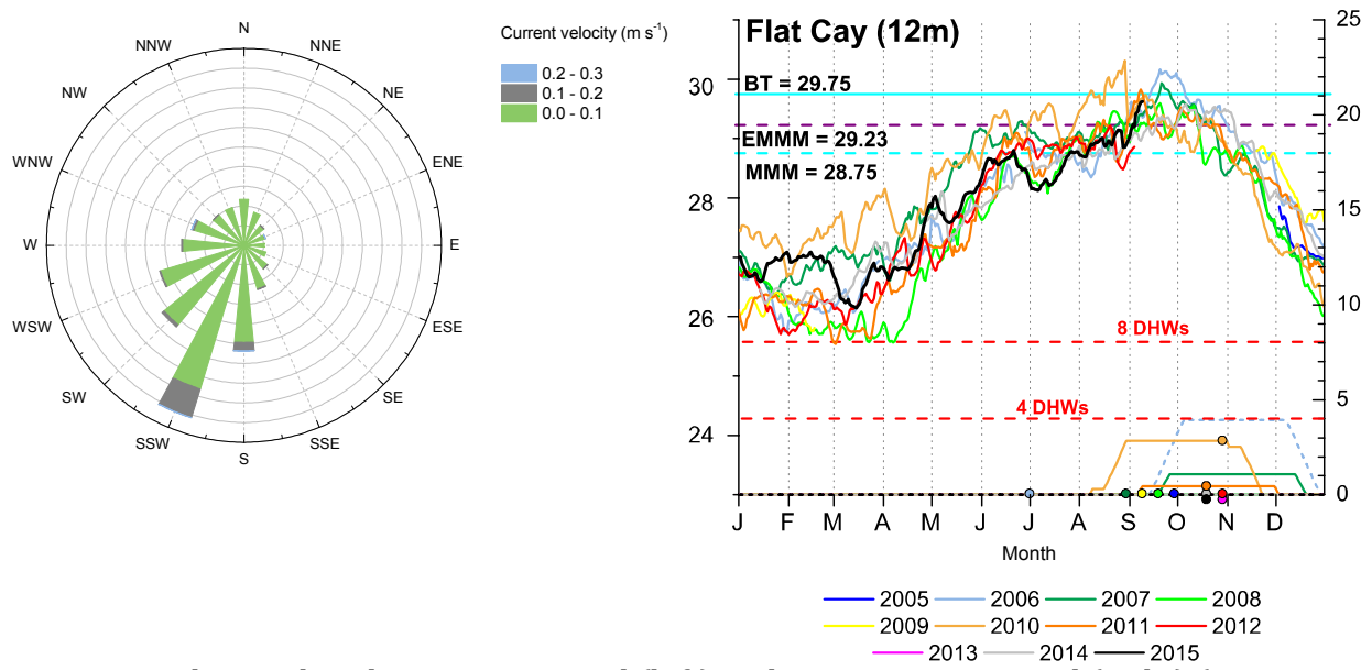
Figure 138. Flat Cay benthic current speed (left) and temperature record (right) (14 m depth).
