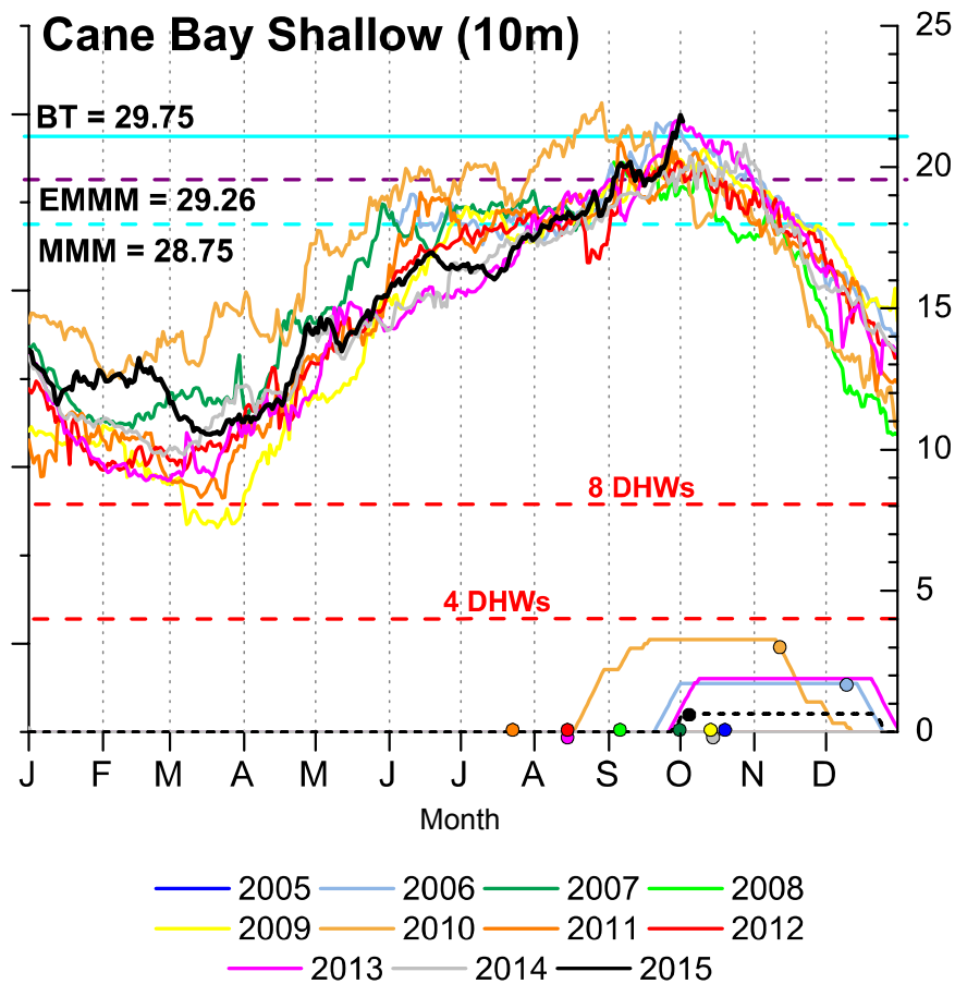
Figure 27. Cane Bay benthic temperatures (8 m depth)
