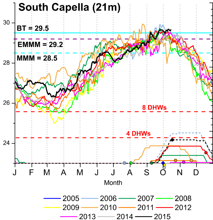
Figure 179. South Capella benthic temperature record (24 m depth).
