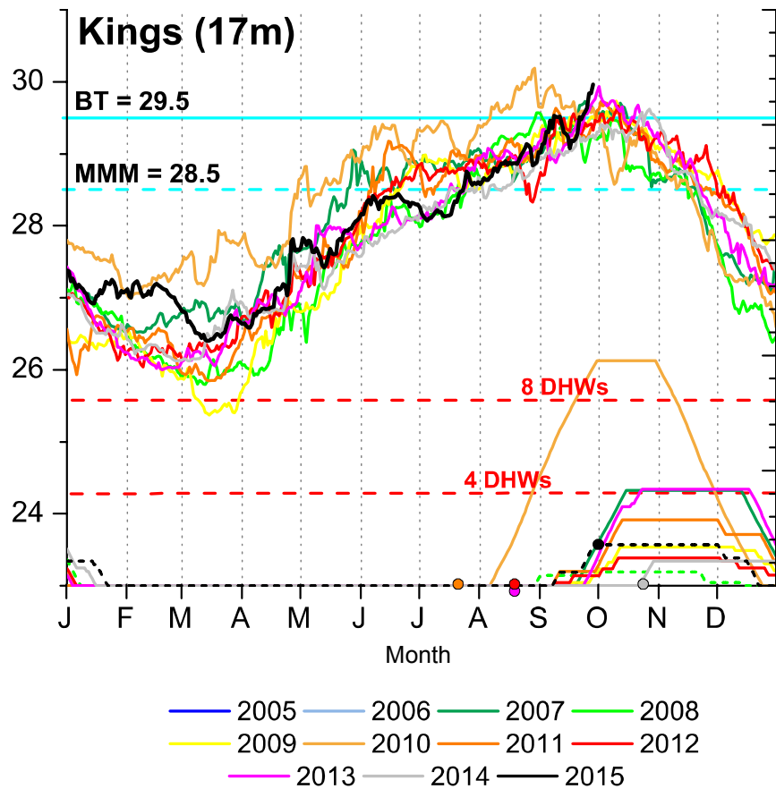
Figure 57. Kings Corner benthic temperature (17 m depth)
