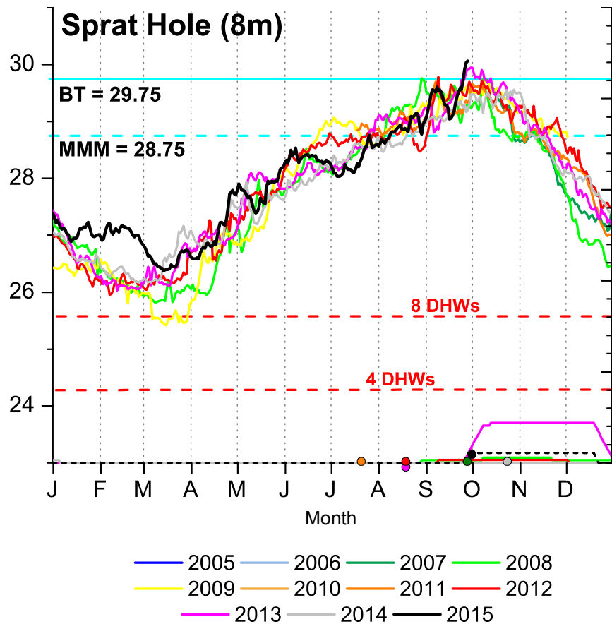
Figure 87. Sprat Hole benthic temperature (7 m depth).
