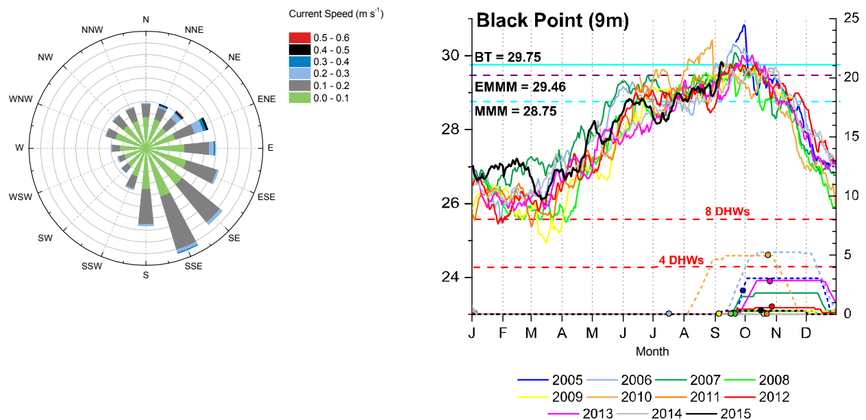
Figure 107. Black point current speed and benthic temperature record (8 m depth).
