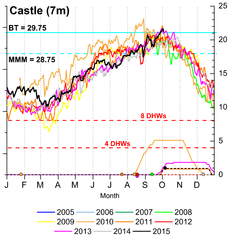
Figure 37. Castle benthic temperatures (9 m depth).
