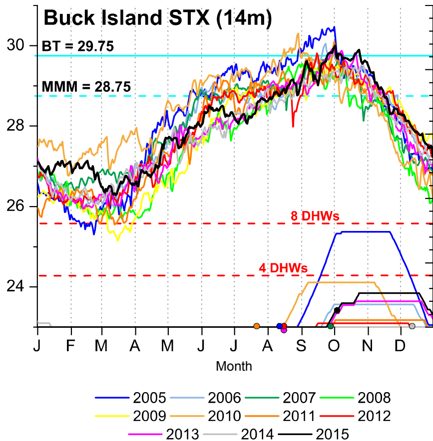
Figure 22. Buck Island, St. Croix benthic temperatures (14 m depth). Data provided by the National Park Service (site BUIS_SFR).
