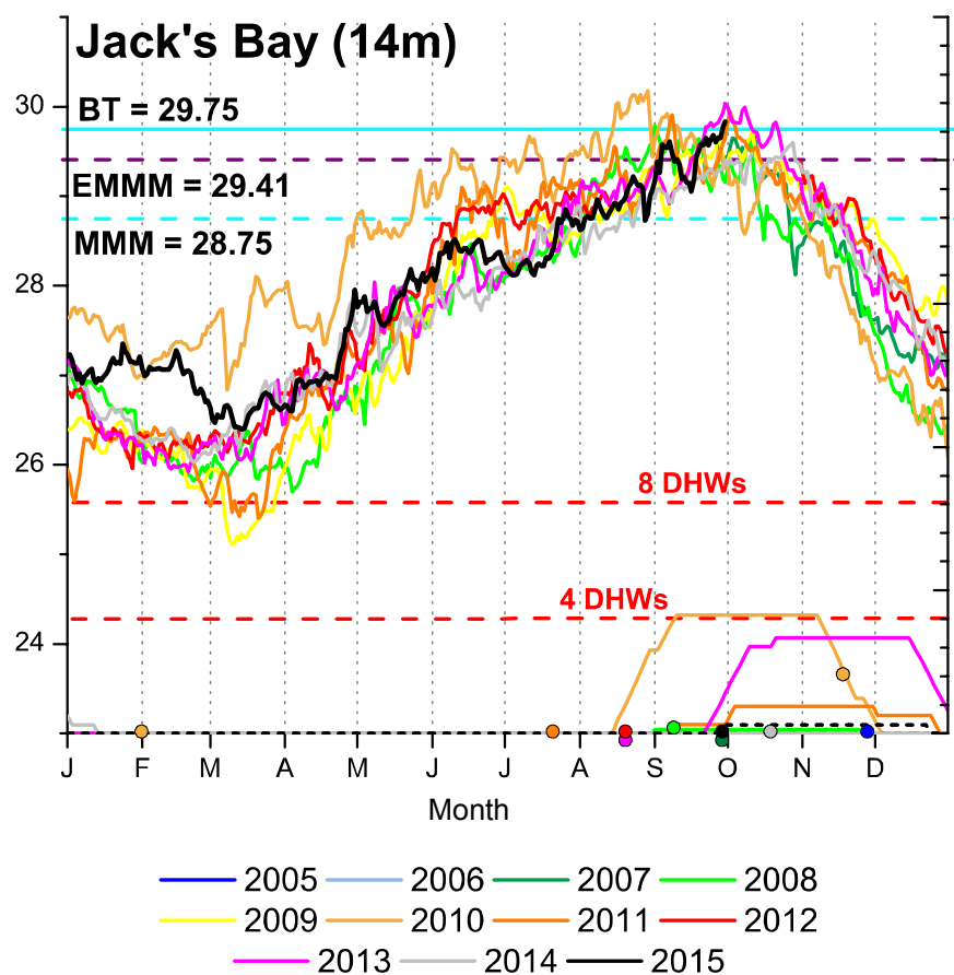
Figure 52. Jacks Bay benthic temperature at 12 m depth
