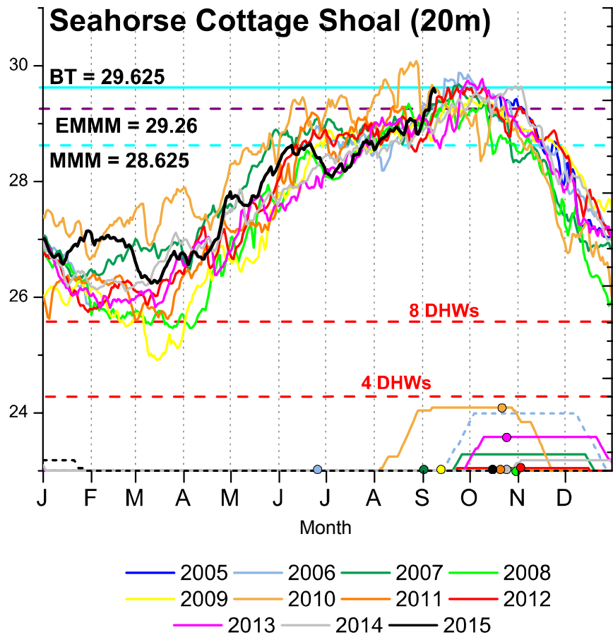
Figure 174. Seahorse benthic temperature record (21 m depth).
