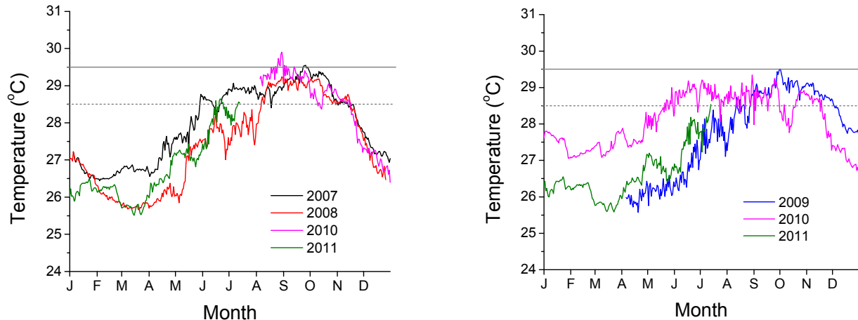
Figure 82. Salt River Deep benthic temperature at 30 m depth (left) and 40 m depth (right).
