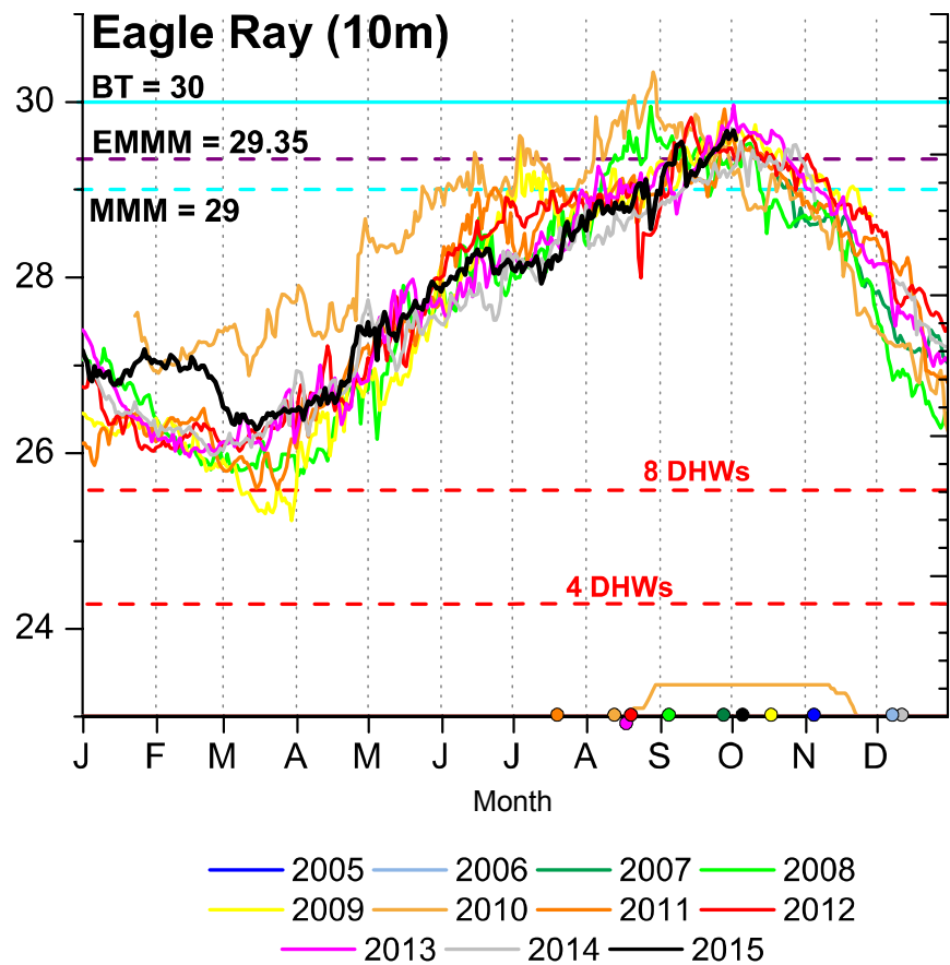
Figure 42. Eagle Ray benthic temperature at 9 m depth
