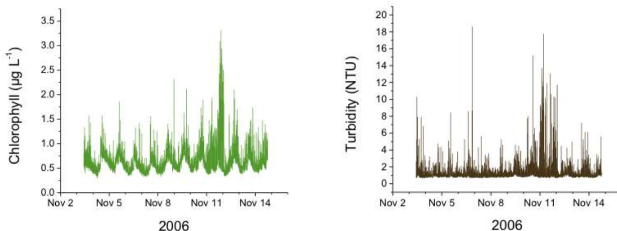
Figure 108. Black Point chlorophyll (left) and turbidity (right) record (16 m depth).
