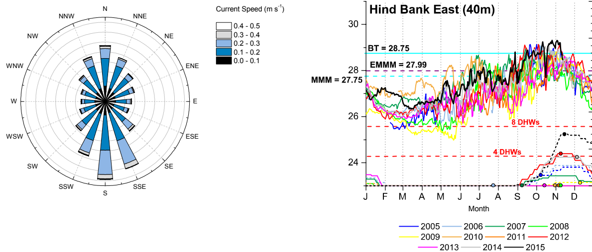
Figure 153. (top) Hind Bank benthic current speed (40m depth). (bottom) Benthic temperature record at 40 m depth.
