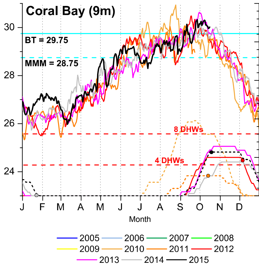
Figure 92. Coral Bay benthic temperature (9 m depth)
