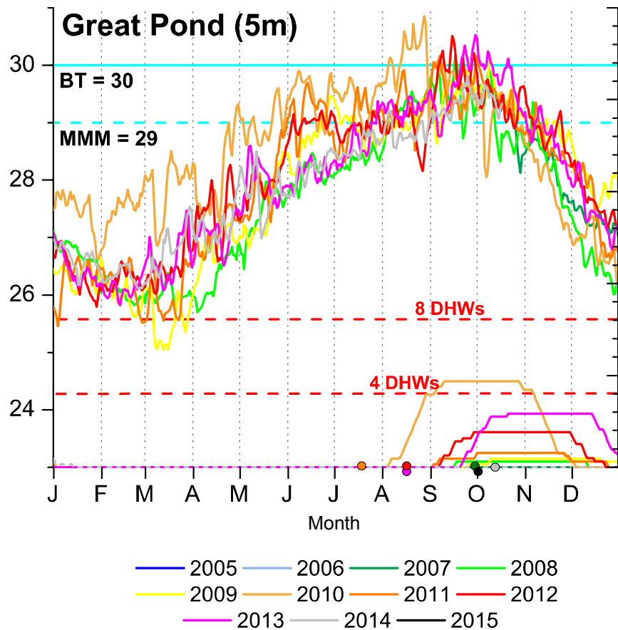
Figure 47. Great Pond benthic temperature (5 m depth).
