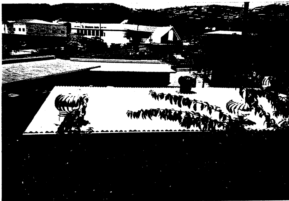
Photo No. 11 - A Corrugated Iron Roof Was Built Over the Soil Pile With Roof Turbines at the Top of the Vent Pipes for Passive Soil Venting
