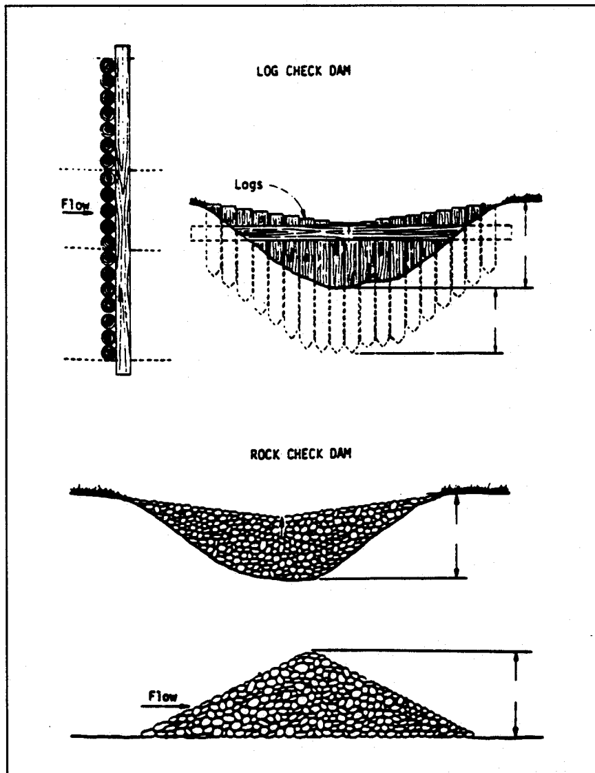
Figure 8. Typical check dams. (Source: Ref. 26)
