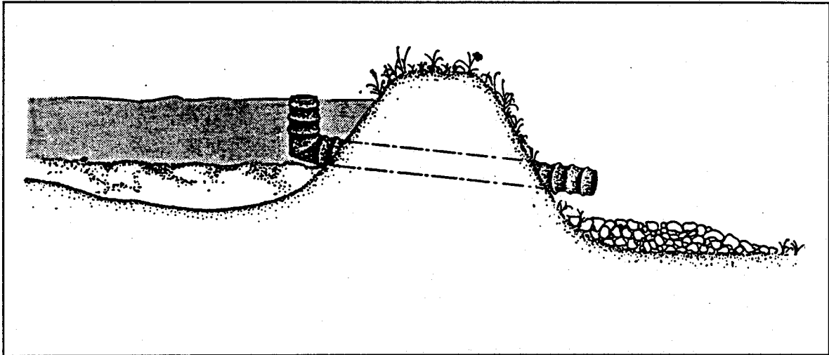
Figure 11. Small sediment basin with outlet pipe discharging on energy dissipator to prevent erosion at discharge end. (Source: Ref. 23)
