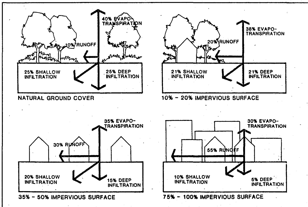
Figure 2. An example of the effects of development on runoff. (Source: Ref. 15)
