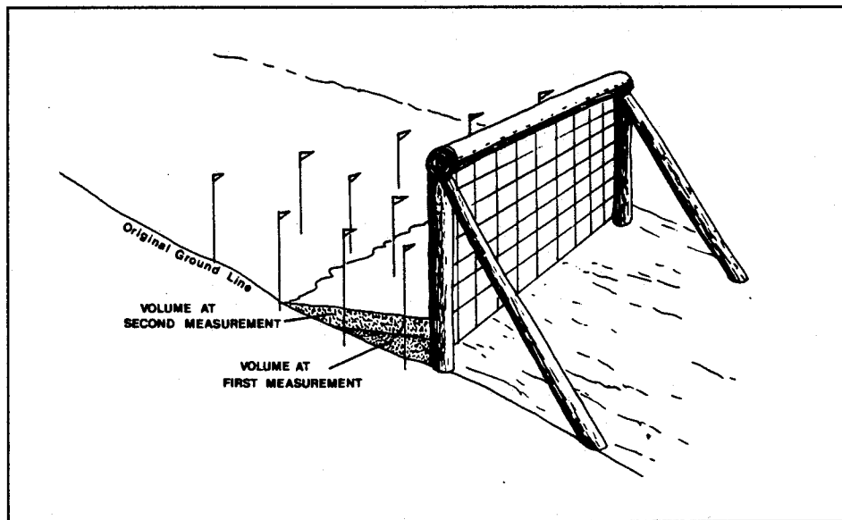
Figure 4. Eroded soil trapped behind fabric dams can be measured periodically to document erosion trends. (Source: Ref. 6)
