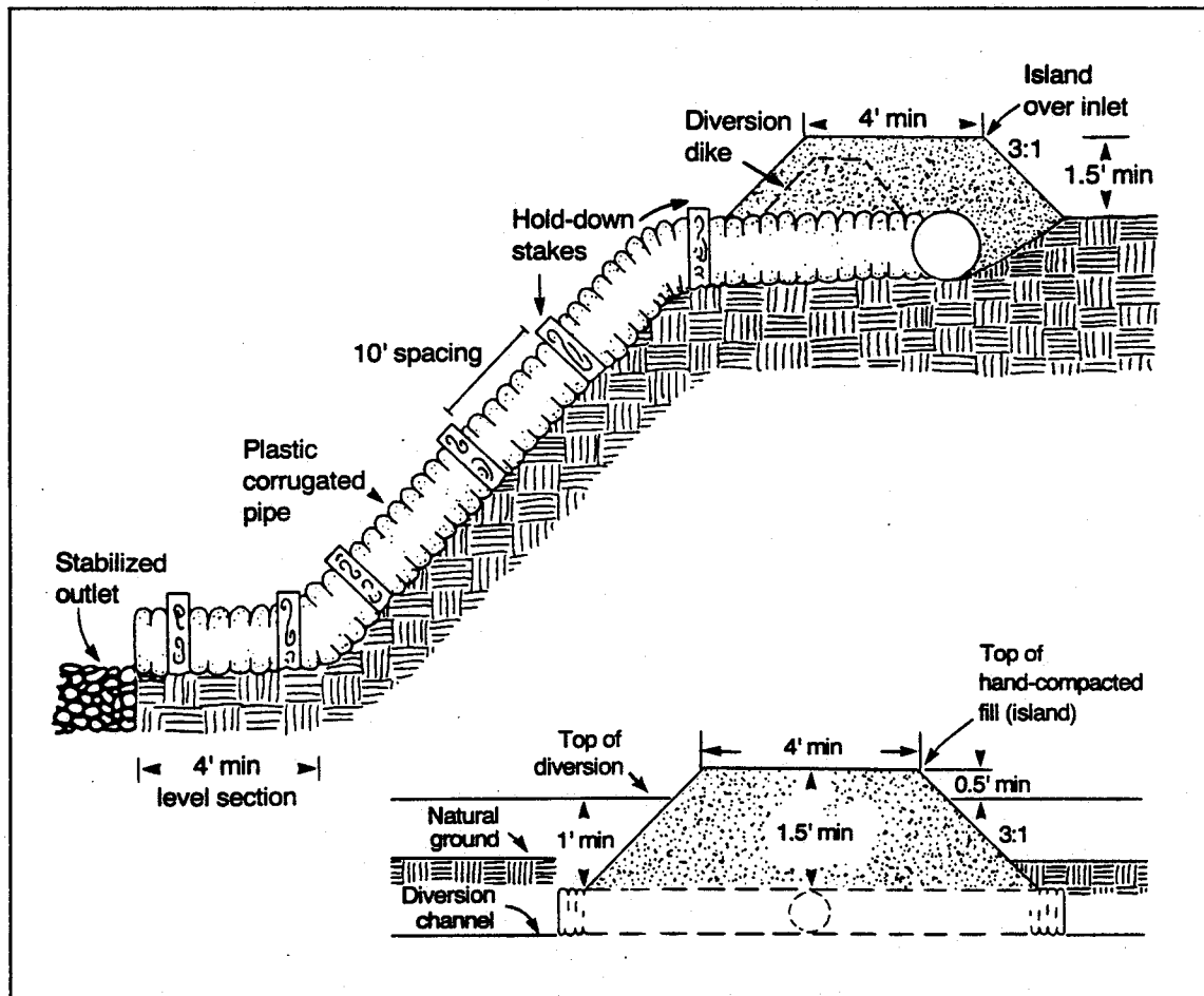
Figure 7. Cross-section of temporary slope drain and detail of inlet. (Source: Ref. 1)
