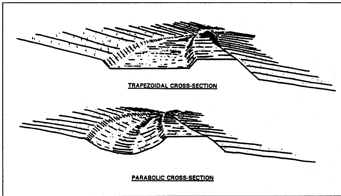
Figure 5. Typical interceptor dikes and swales. (Source: Ref. 26)
