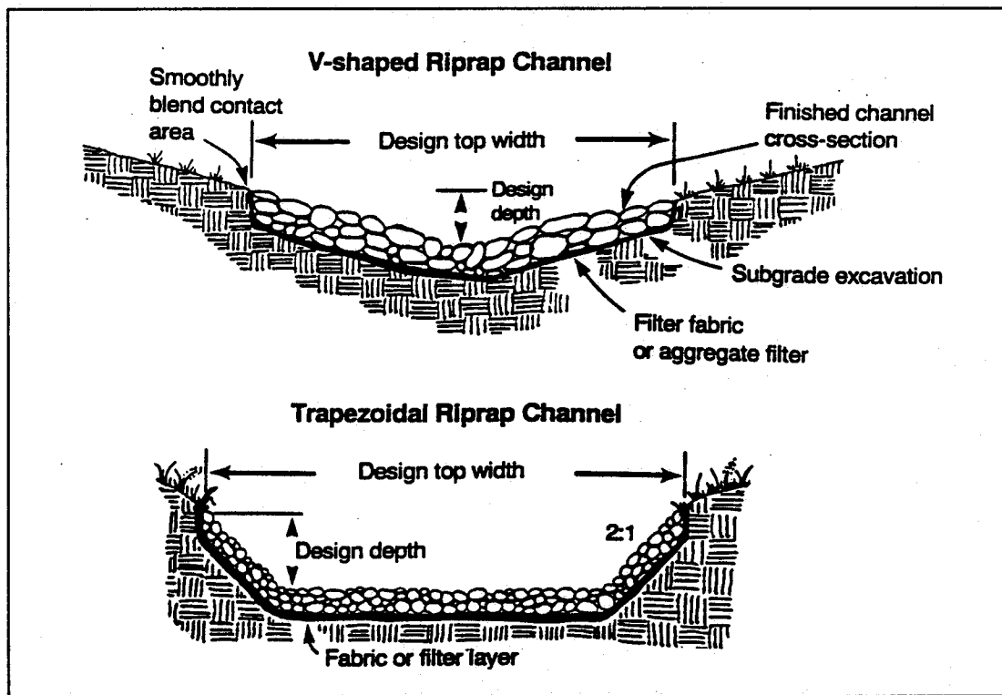
Figure 6. Typical riprap-lined channel cross-sections. (Source: Ref. 1)
