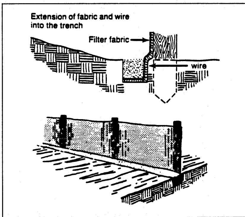
Figure 10. Sediment fence details. (Source: Ref. 26)
