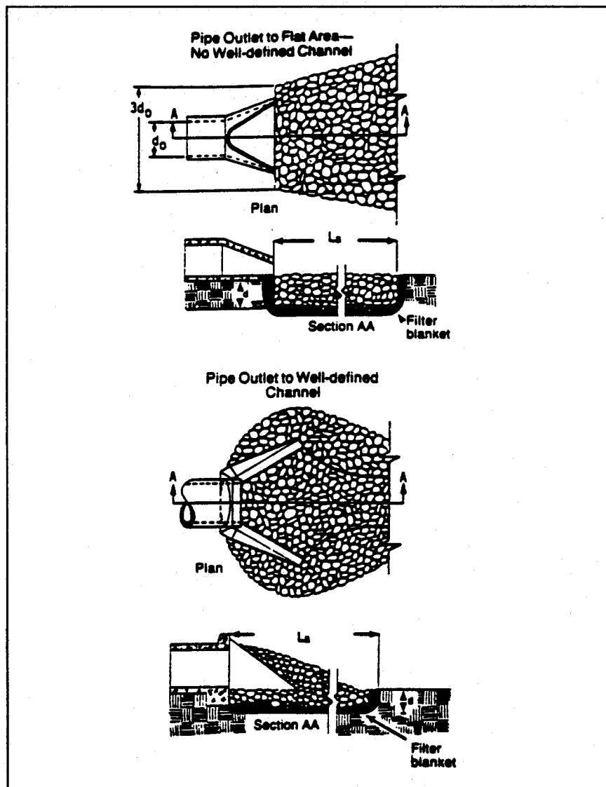
Figure 9. Typical details for rock outlet protection. (Source: Ref. 26)
