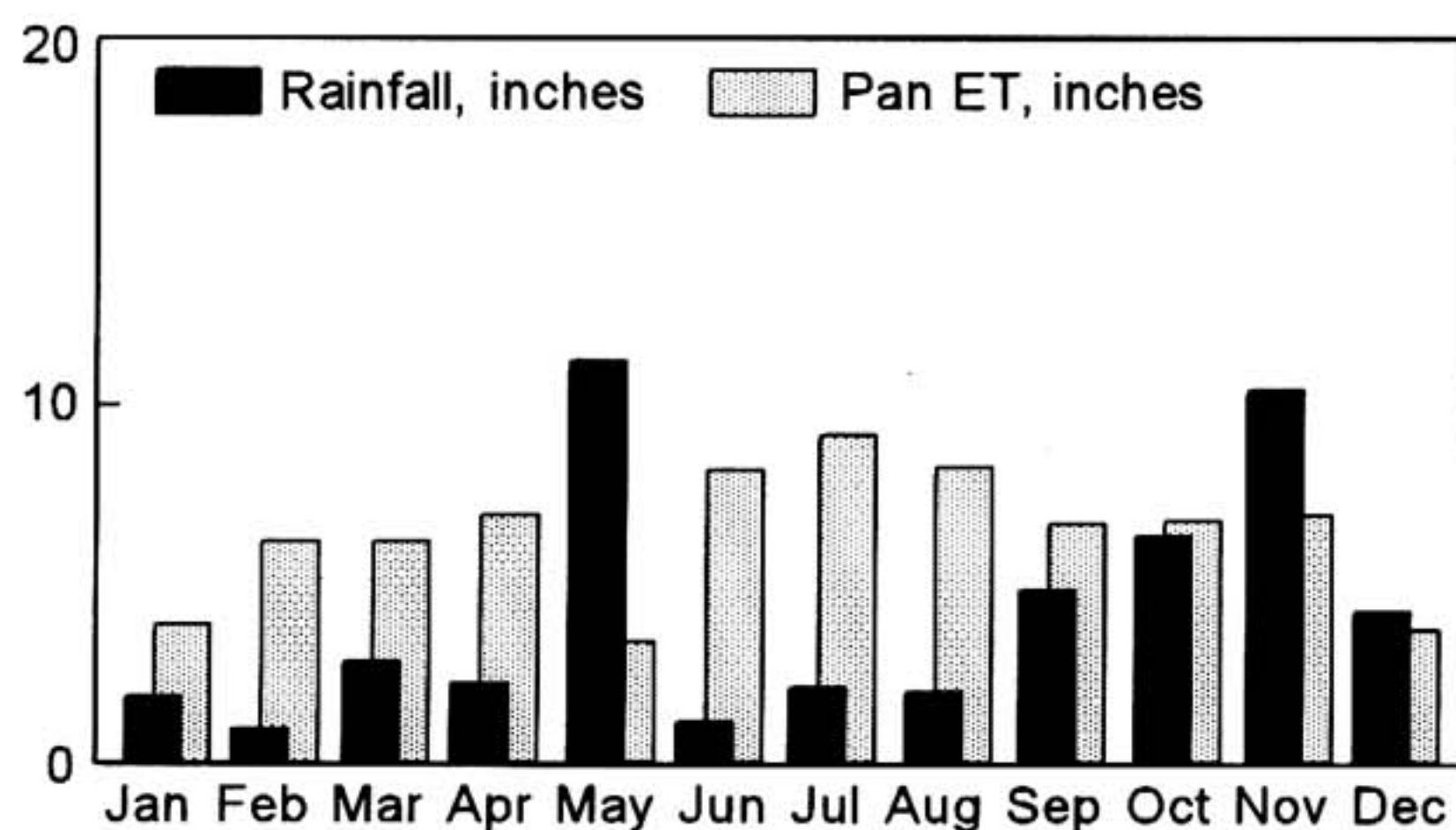
Figure 1. Rainfall and potential evapotranspiration at UVI-AES, 1992.
