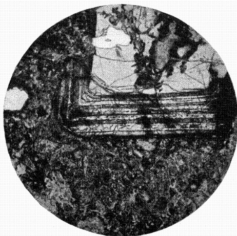
FIG. 6.— Augite porphyrite showing zoned augite crystal set in fine-grained groundmass Taken in plain light, magnified about 30 times. K. S. 6, Mayaguez-Consumo-Maricao road.
